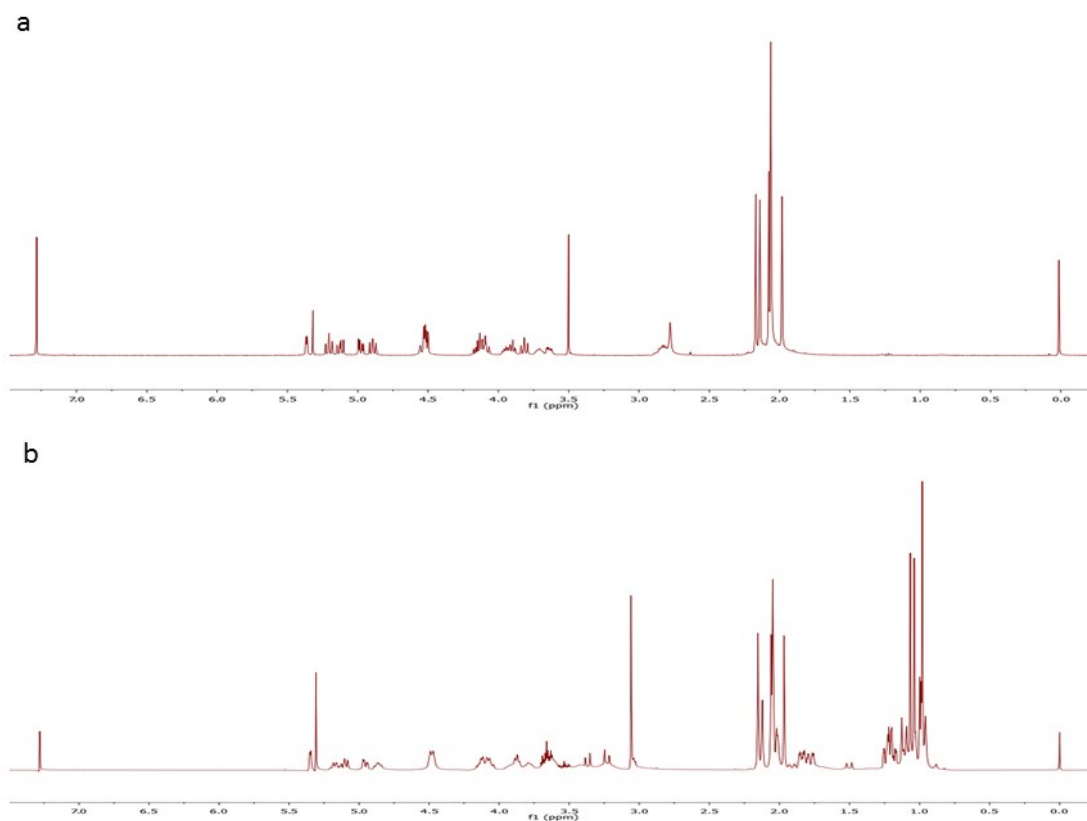
Figure S1. ^1\text{H} NMR spectra of (a) lactose containing diamine and (b) the prepolymer with isophorone diisocyanate.
