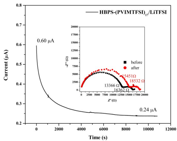
Figure S 1 Chronoamperometry curves and impedance spectra of the HBPS-(PVIMTFSI) 17 /LiTFSI electrolyte obtained at 30°C
