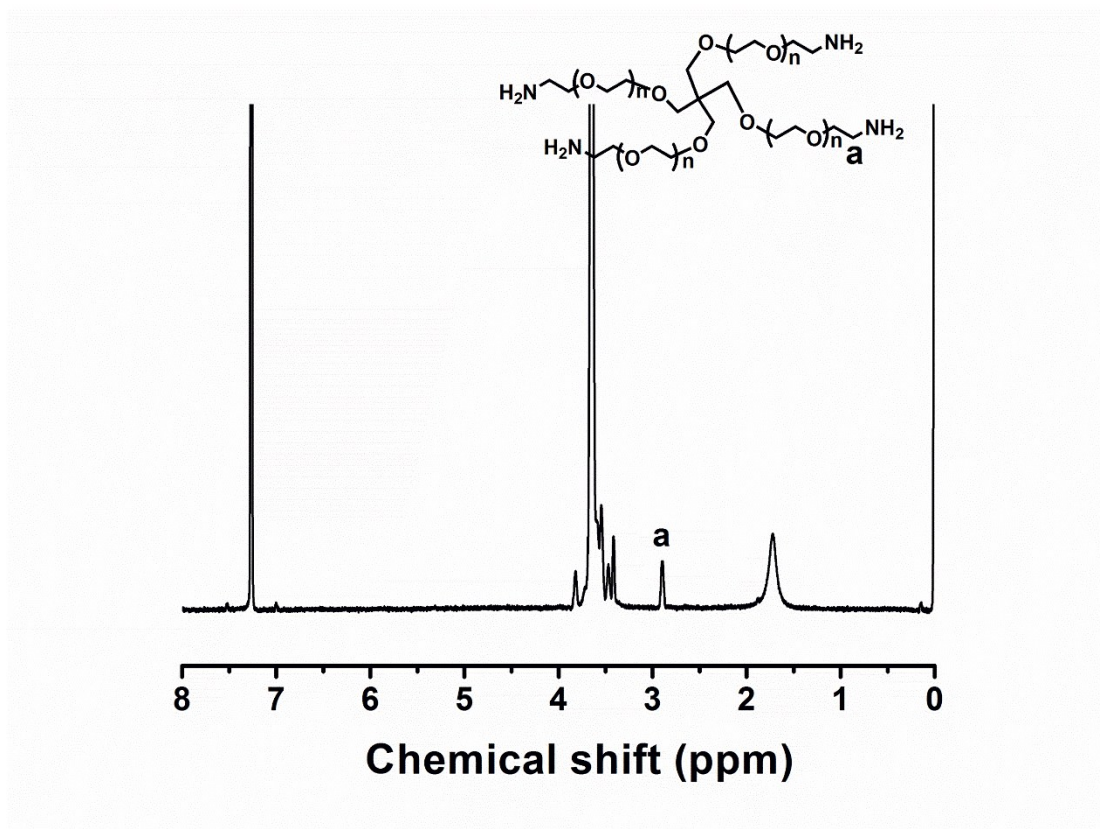
Figure S1 The ^1\text{H-NMR} spectrum of 4-arm-PEG-NH 2 in CDCl 3 .
