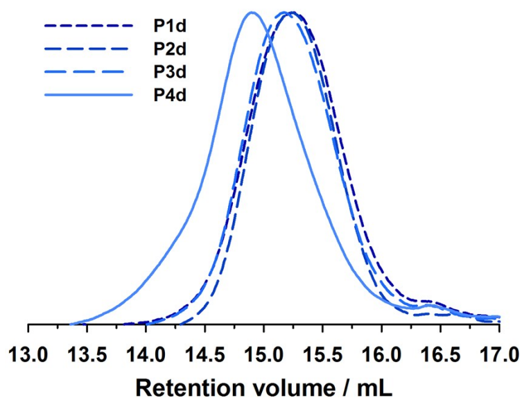
Figure S4. Size exclusion chromatograms ( \text{CHCl}_3 eluent, 1 \text{ mL} \cdot \text{min}^{-1} ) of CdA-digly-PSqMA P1d–P4d after deprotection and precipitation.
