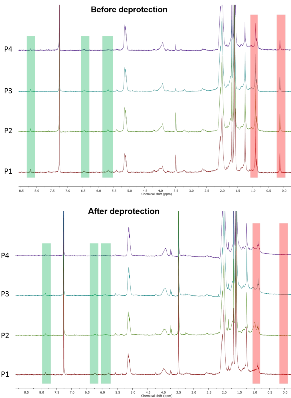
Figure S2. 1 H NMR spectra in CDCl 3 of P1–P4 before (top) and after (bottom) deprotection. The green color areas show the protons from the cladribine group and the red color areas show the TBDMS group.
