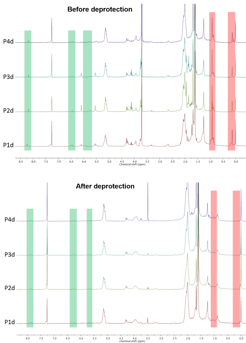
Figure S1. 1 H NMR spectra in CDCl 3 of P1d–P4d before (top) and after (bottom) deprotection. The green color areas show the protons from the cladribine group and the red color areas show the TBDMS group.
