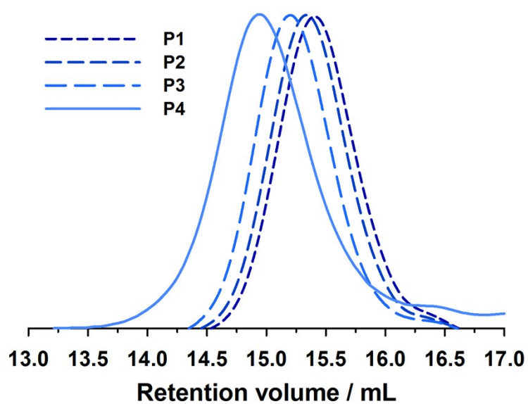
Figure S3. Size exclusion chromatograms ( \text{CHCl}_3 eluent, 1 \text{ mL} \cdot \text{min}^{-1} ) of CdA-PSqMA P1–P4 after deprotection and precipitation.
