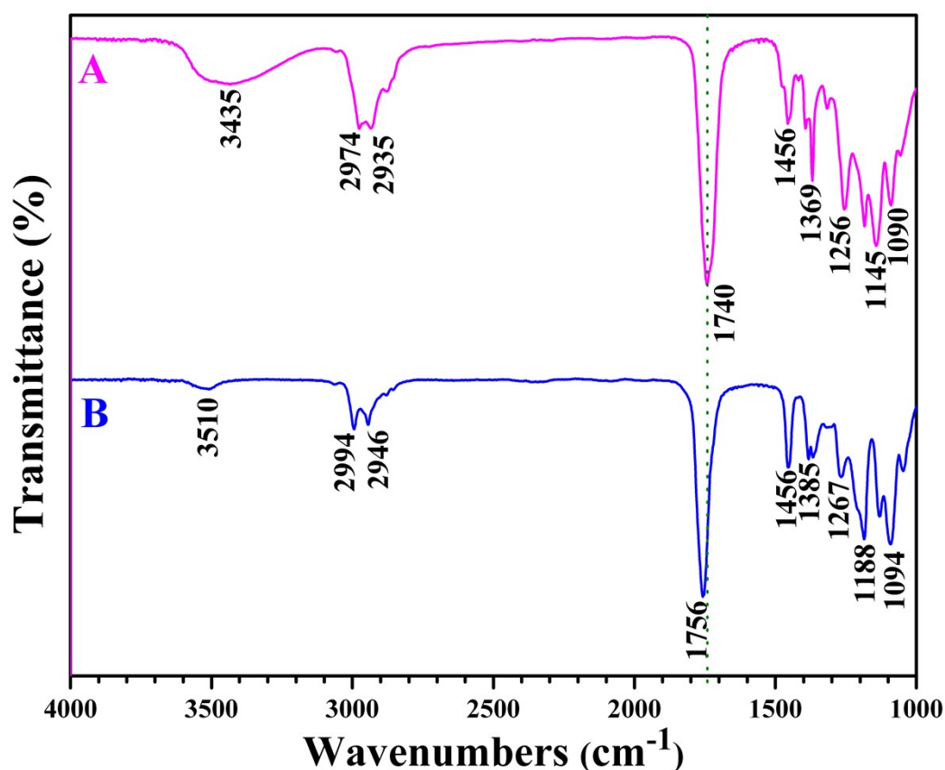
Figure S1. FT-IR spectra of PtBHBMA 1 (A) and PtBA-g-PLA 2 (B).
