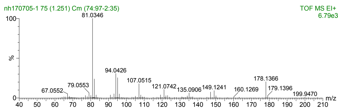
Fig S2 Mass spectrum of 8-furyl-1-octene
