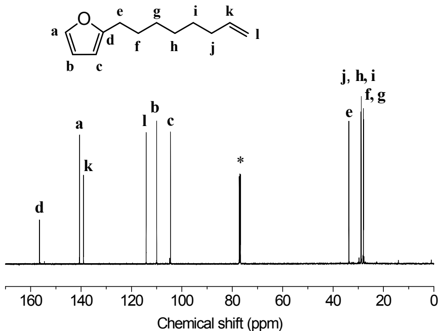
Fig S1 ^{13}\text{C} -NMR spectrum of 8-furyl-1-octene (Solvent: chloroform- d ; temp.: 20°C)
