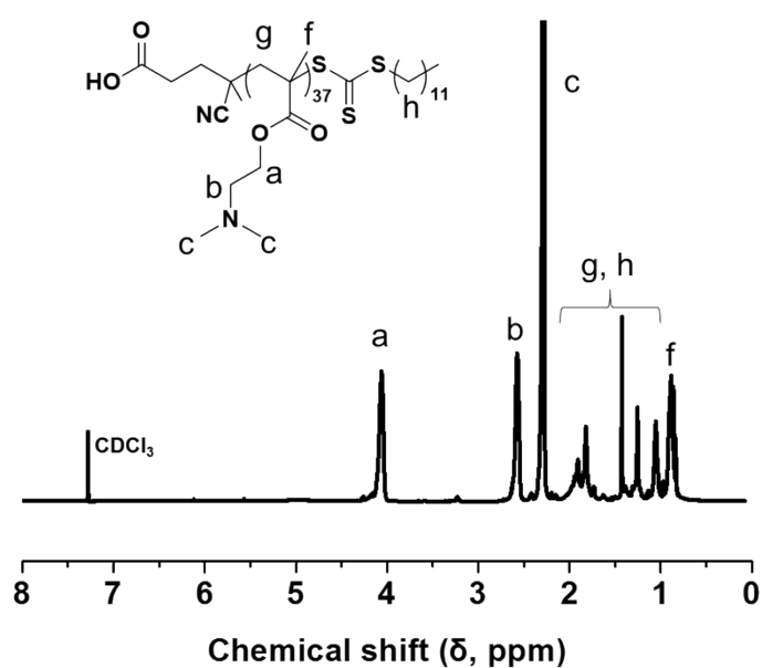
Figure S1. 1 H NMR spectrum of PDMA 37 macro CTA (recorded in CDCl 3 ).
