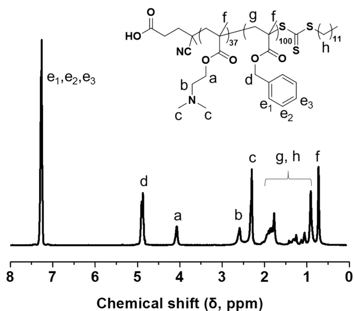
Figure S2. ^1\text{H} NMR spectrum of PDMA 37 - b -PBzMA 96 block copolymer (recorded in CDCl 3 ).
