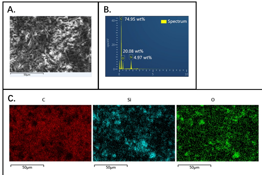
Figure S3. Tablet compressing Backscattered electron images of 3D hierarchical porous monoliths (A), Element composition (B) and their corresponding EDX elemental maps (C).
