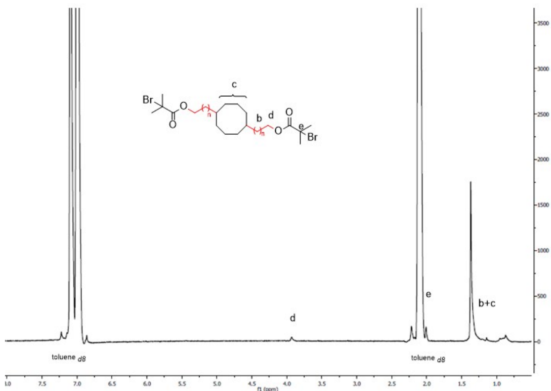
Figure S1. 1 H NMR spectrum of α,ω-dibromo polyethylene
