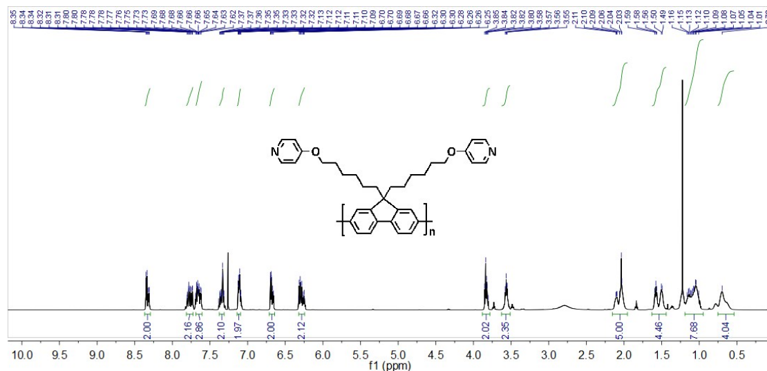
Figure S1. 1 H NMR spectrum of PFPy.
