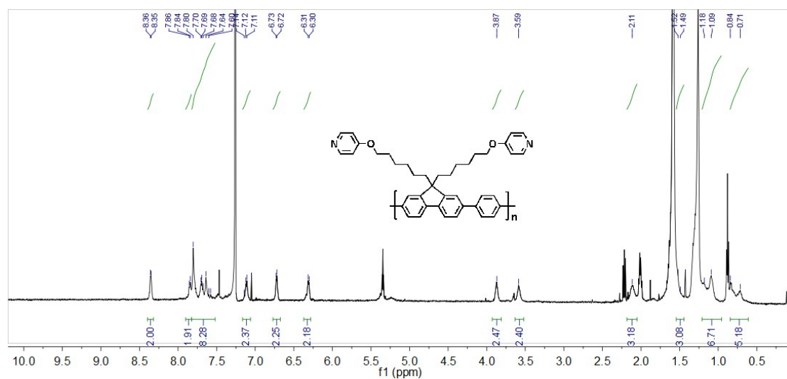
Figure S4. 1 H NMR spectrum of PFPy-P.
