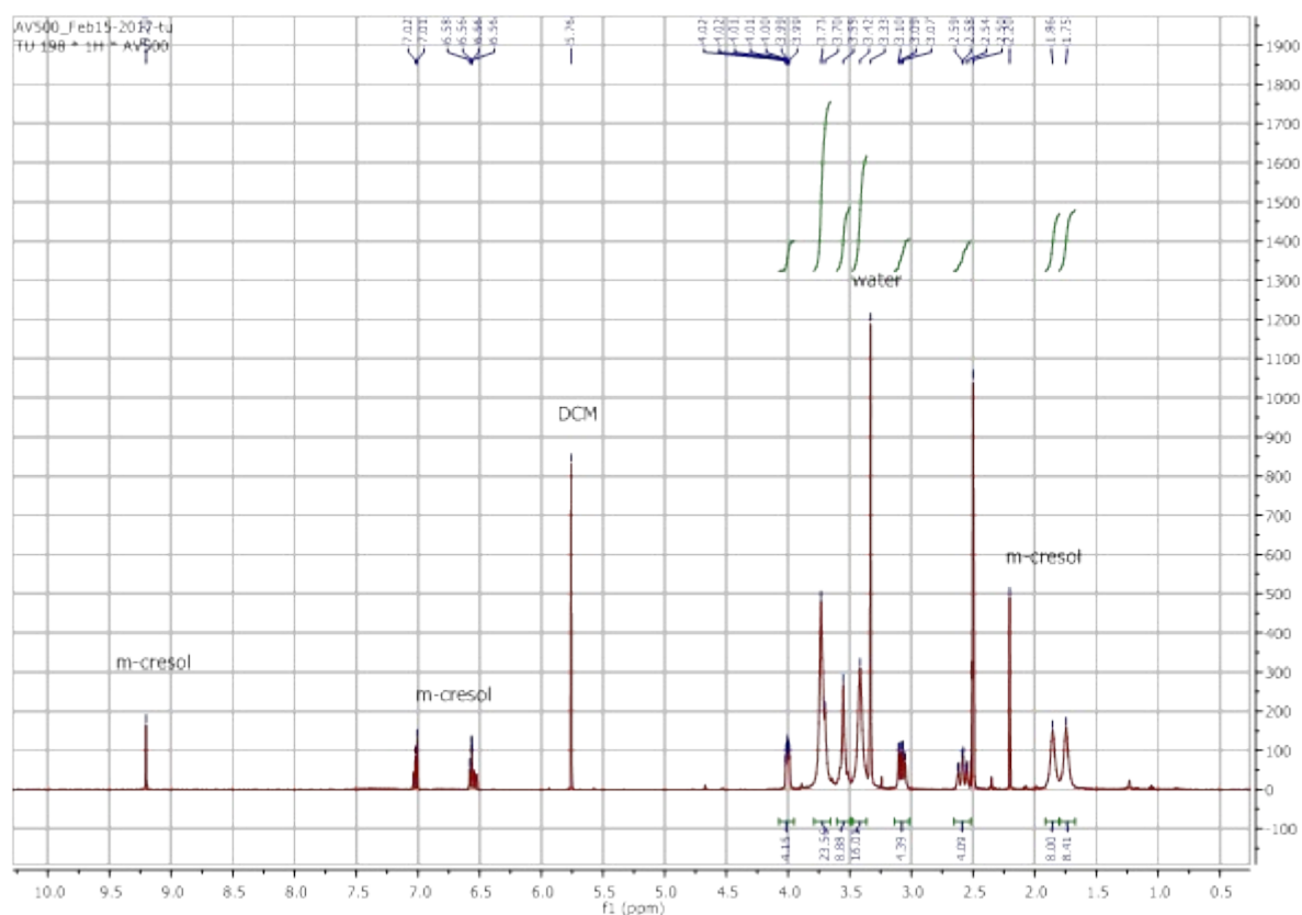
Figure 11: ^1\text{H} -NMR spectrum of PIS-1.
