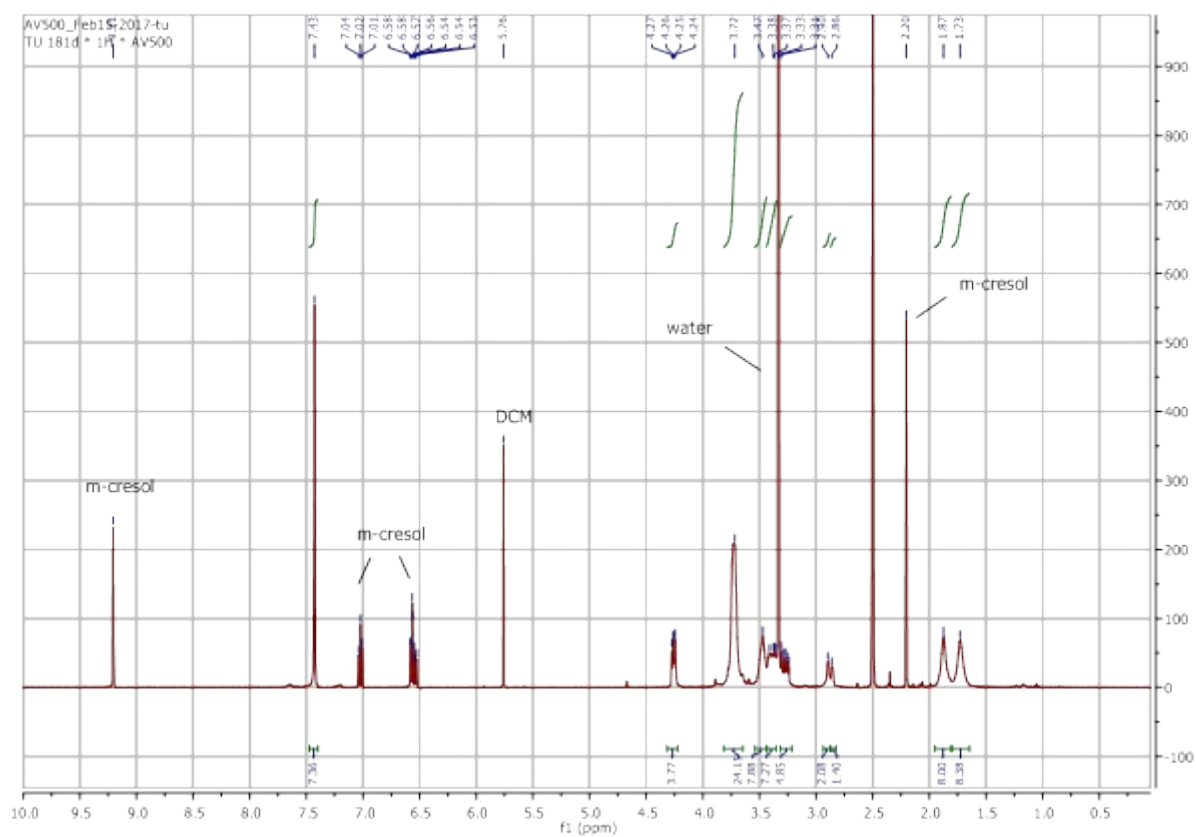
Figure 13: ^1\text{H} -NMR spectrum of PIS-2.
