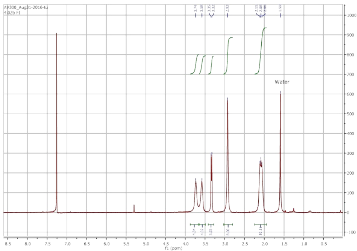
Figure 7: ^1\text{H} -NMR spectrum of 6 .
