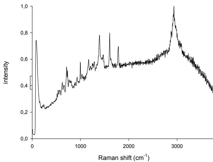
Figure 21: Raman spectrum of PIS-2 .
