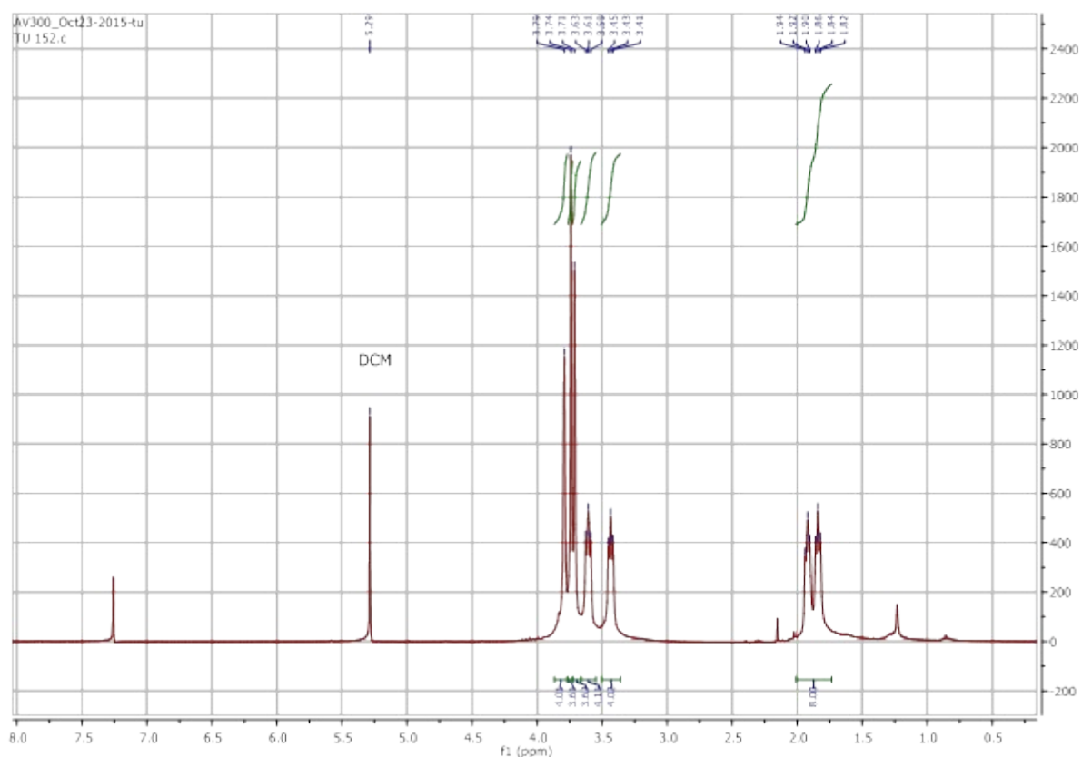
Figure 9: ^1\text{H} -NMR spectrum of 7 .
