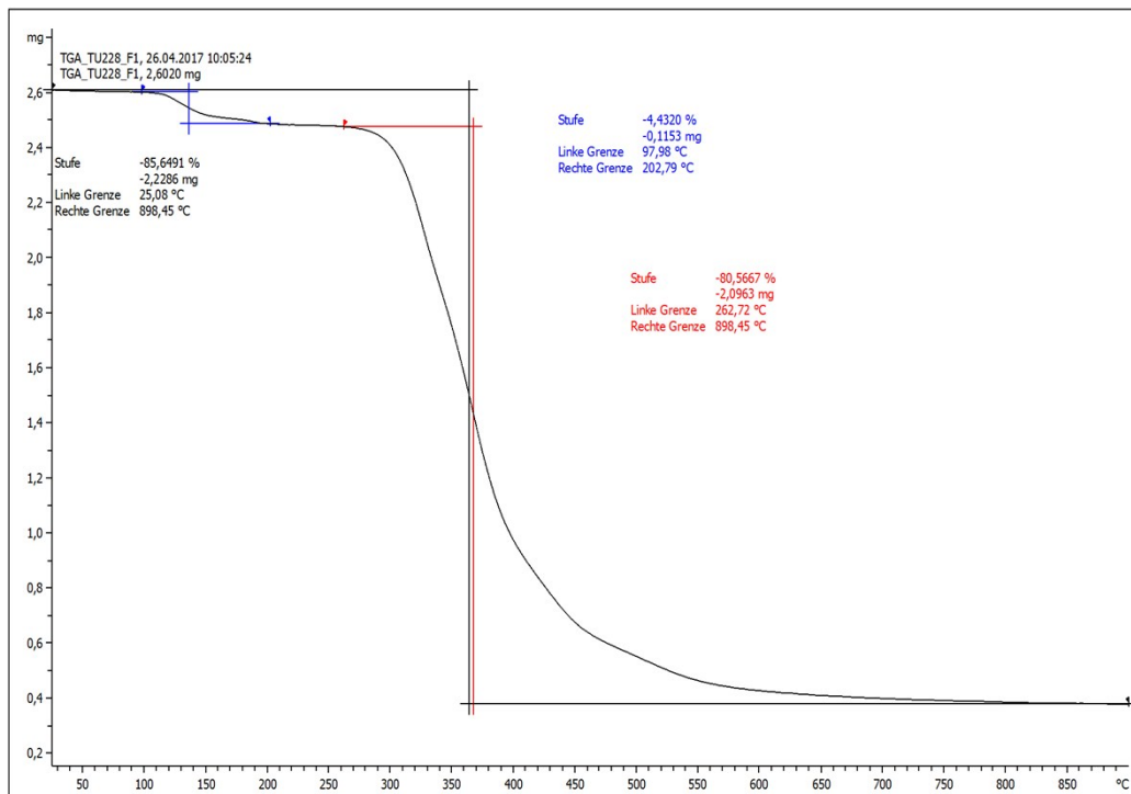
Figure 26: TGA curve of PIS-3.
