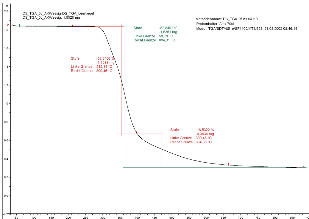
Figure 27: TGA curve of PIS-4.
