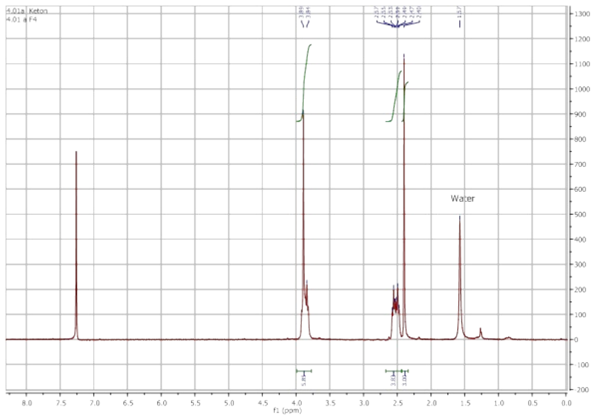
Figure 5: ^1\text{H} -NMR spectrum of 5 .
