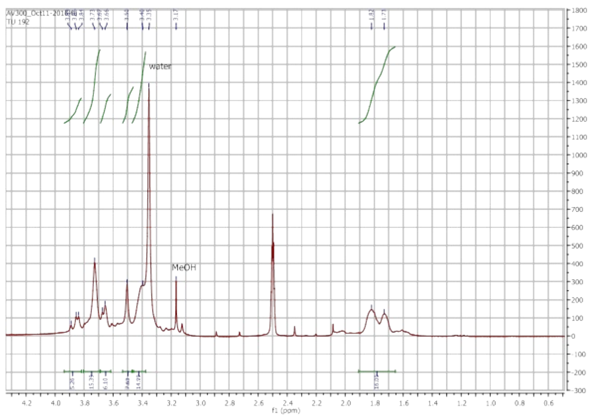
Figure 19: ^1\text{H} -NMR spectrum of PS-1.
