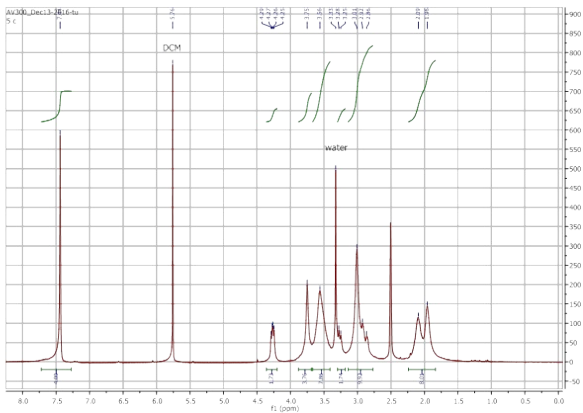
Figure 17: ^1\text{H} -NMR spectrum of PIS-4.
