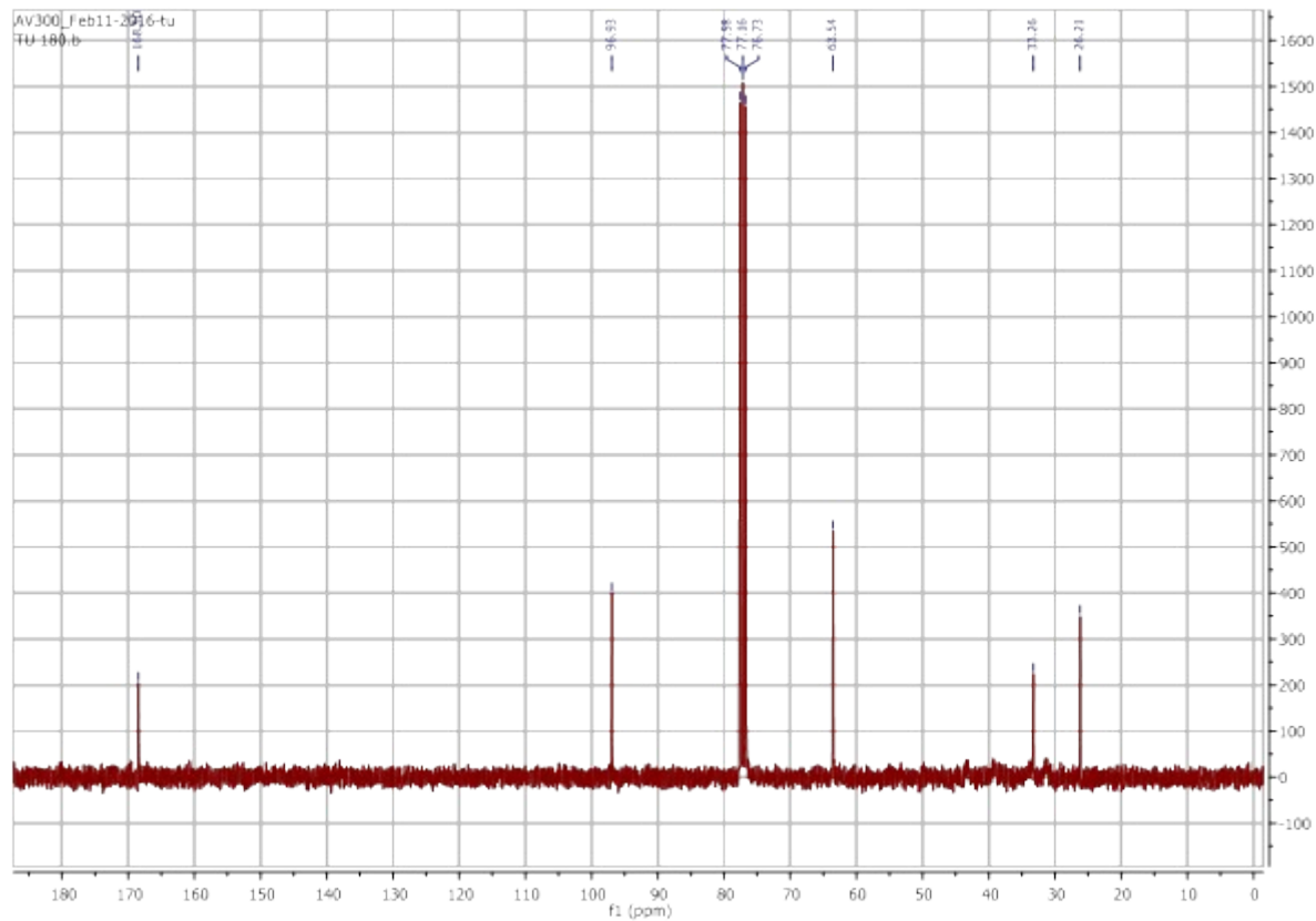
Figure 4: ^{13}\text{C} -NMR spectrum of 3 .
