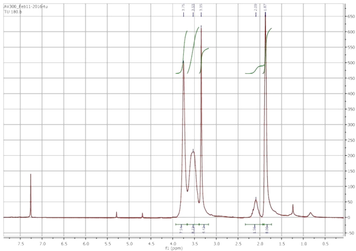
Figure 3: ^1\text{H} -NMR spectrum of 3 .
