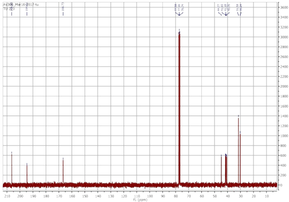
Figure 6: ^{13}\text{C} -NMR spectrum of 5 .
