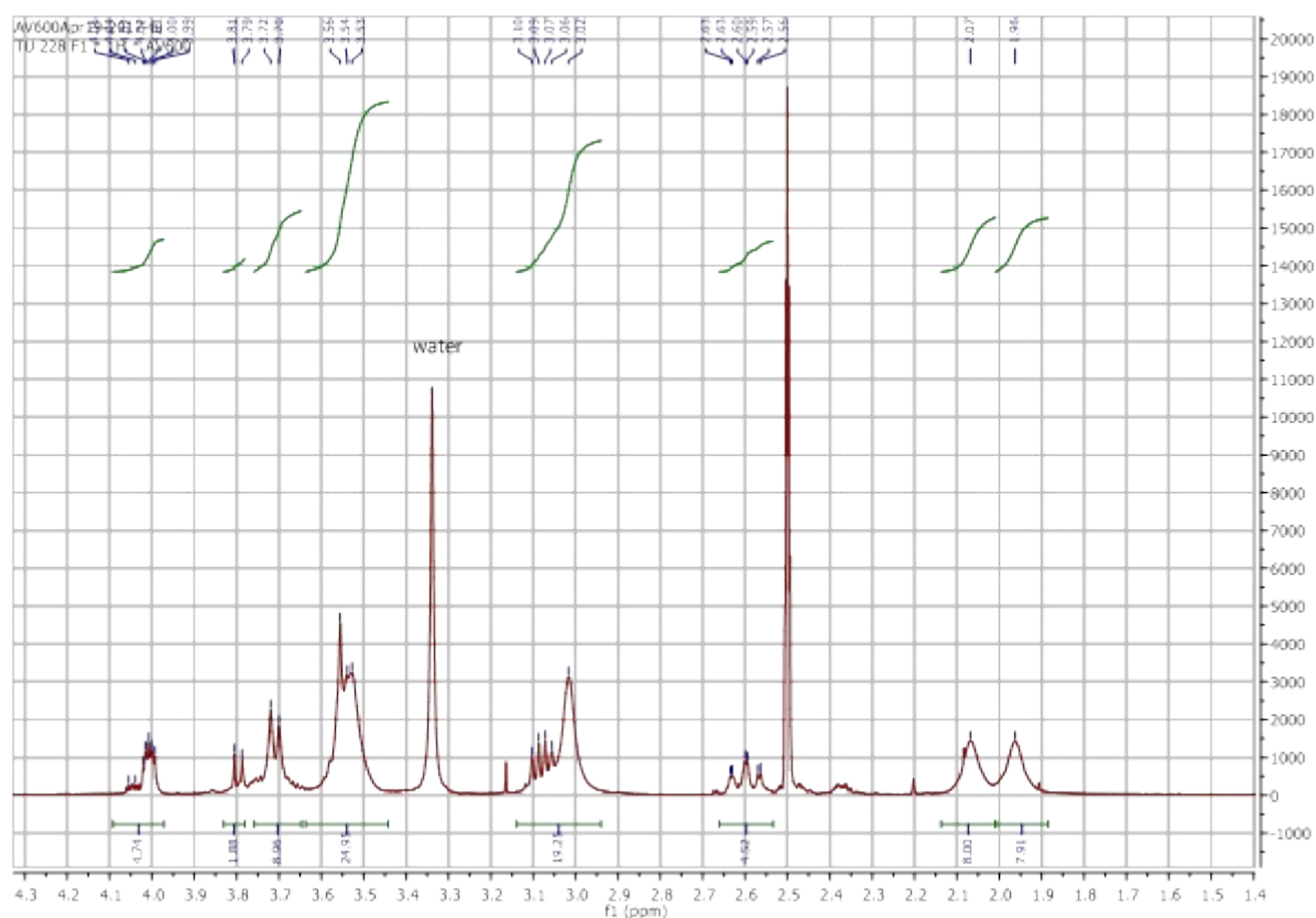
Figure 15: ^1\text{H} -NMR spectrum of PIS-3.
