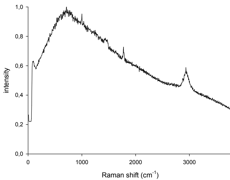
Figure 20: Raman spectrum of PIS-1 .
