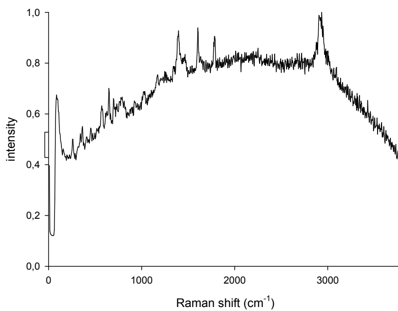
Figure 22: Raman spectrum of PIS-4 .
