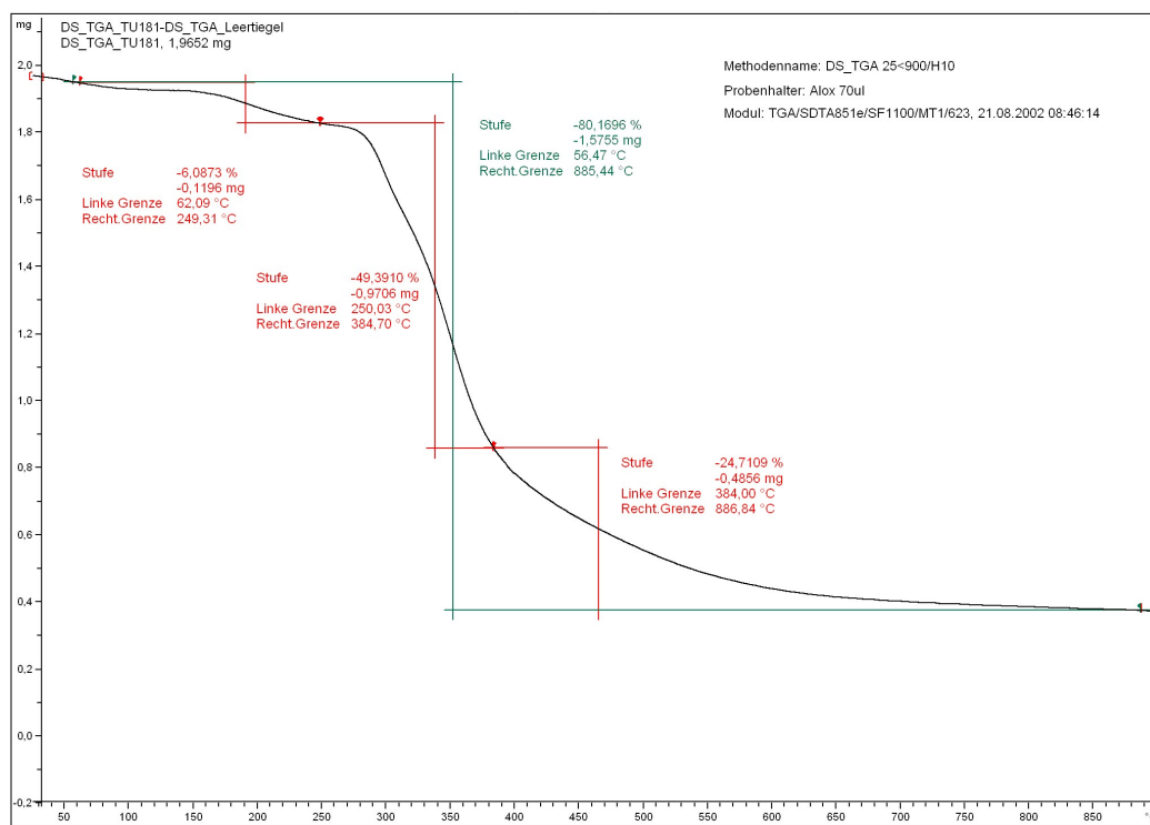
Figure 25: TGA curve of PIS-2.
