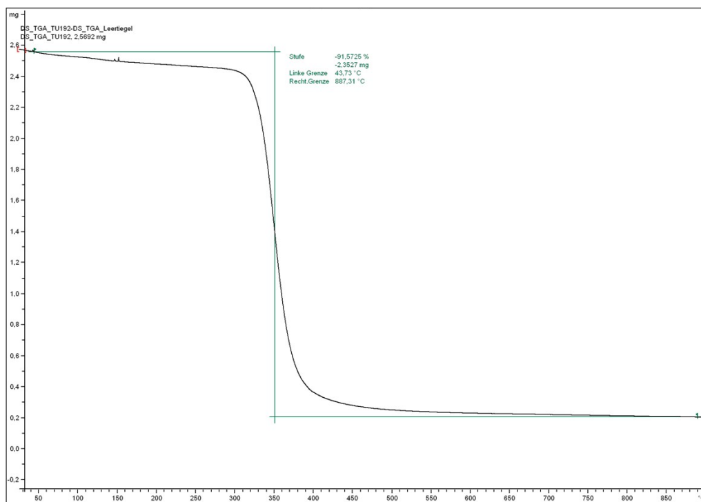
Figure 28: TGA curve of PS-1 .
