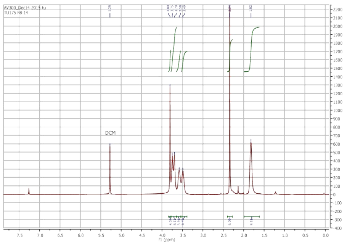
Figure 1: ^1\text{H} -NMR spectrum of 2 .
