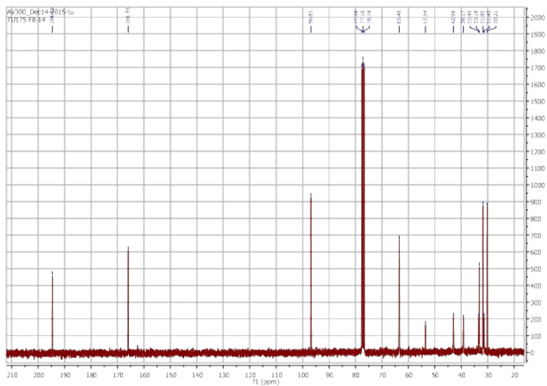
Figure 2: ^{13}\text{C} -NMR spectrum of 2 .
