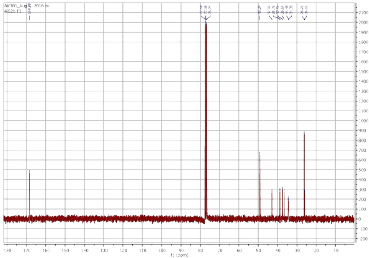
Figure 8: ^{13}\text{C} -NMR spectrum of 6 .
