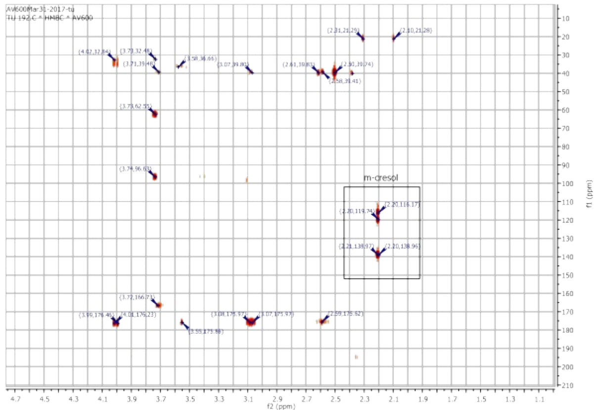
Figure 12: HMBC spectrum of PIS-1.
