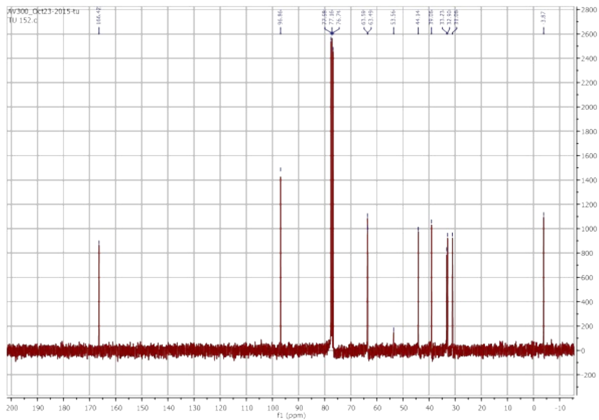
Figure 10: ^{13}\text{C} -NMR spectrum of 7 .
