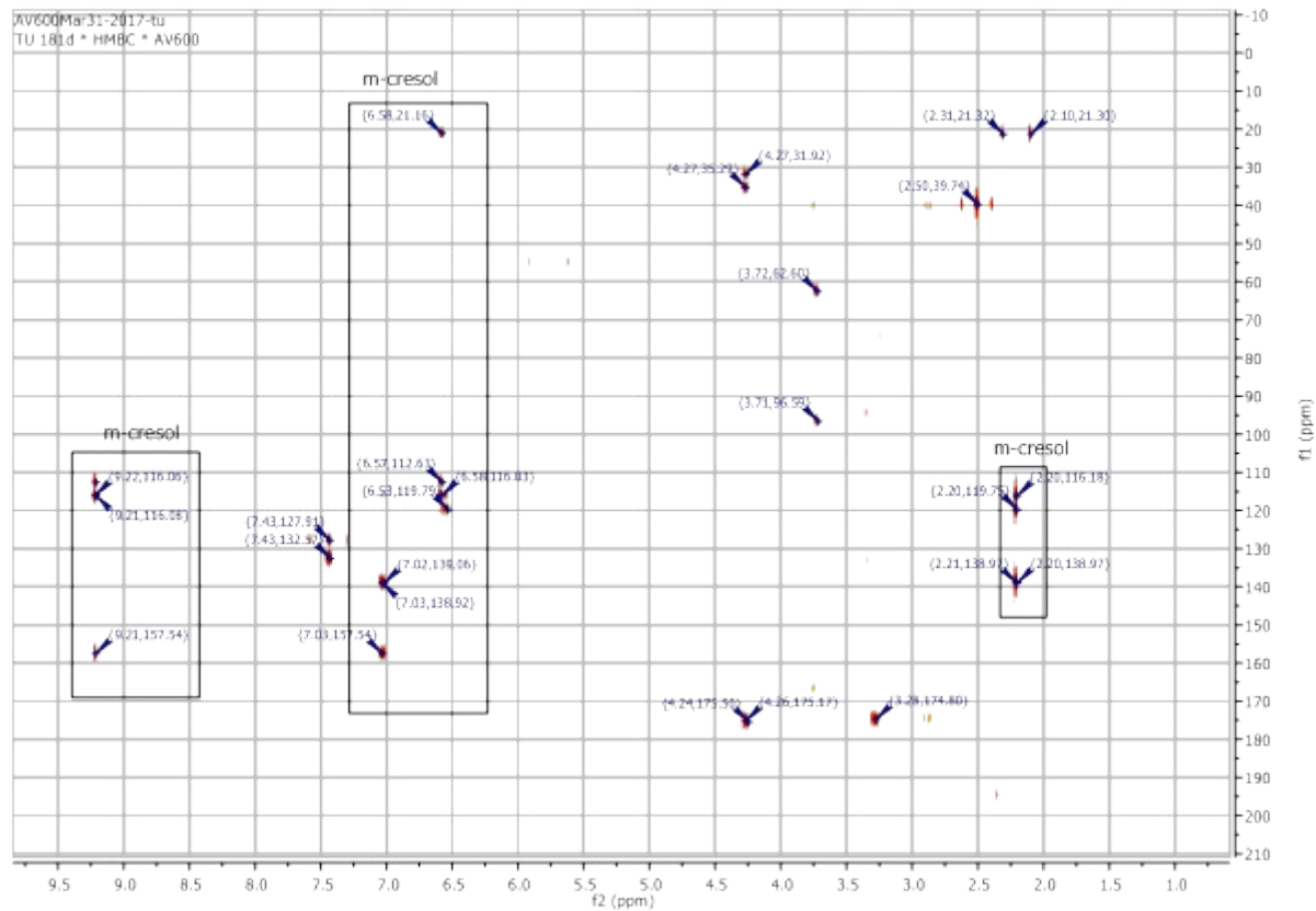
Figure 14: HMBC spectrum of PIS-2.
