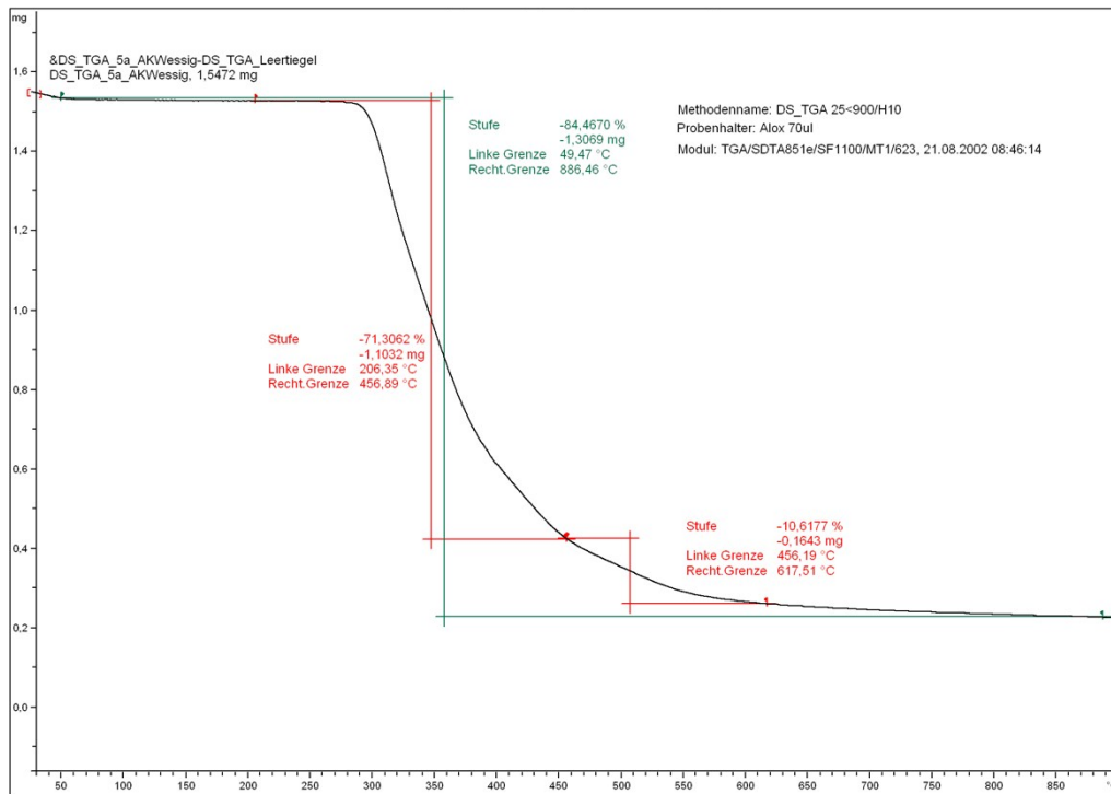
Figure 24: TGA curve of PIS-1.
