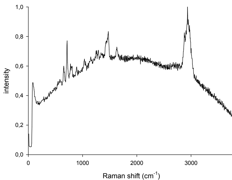
Figure 23: Raman spectrum of PS-1 .
