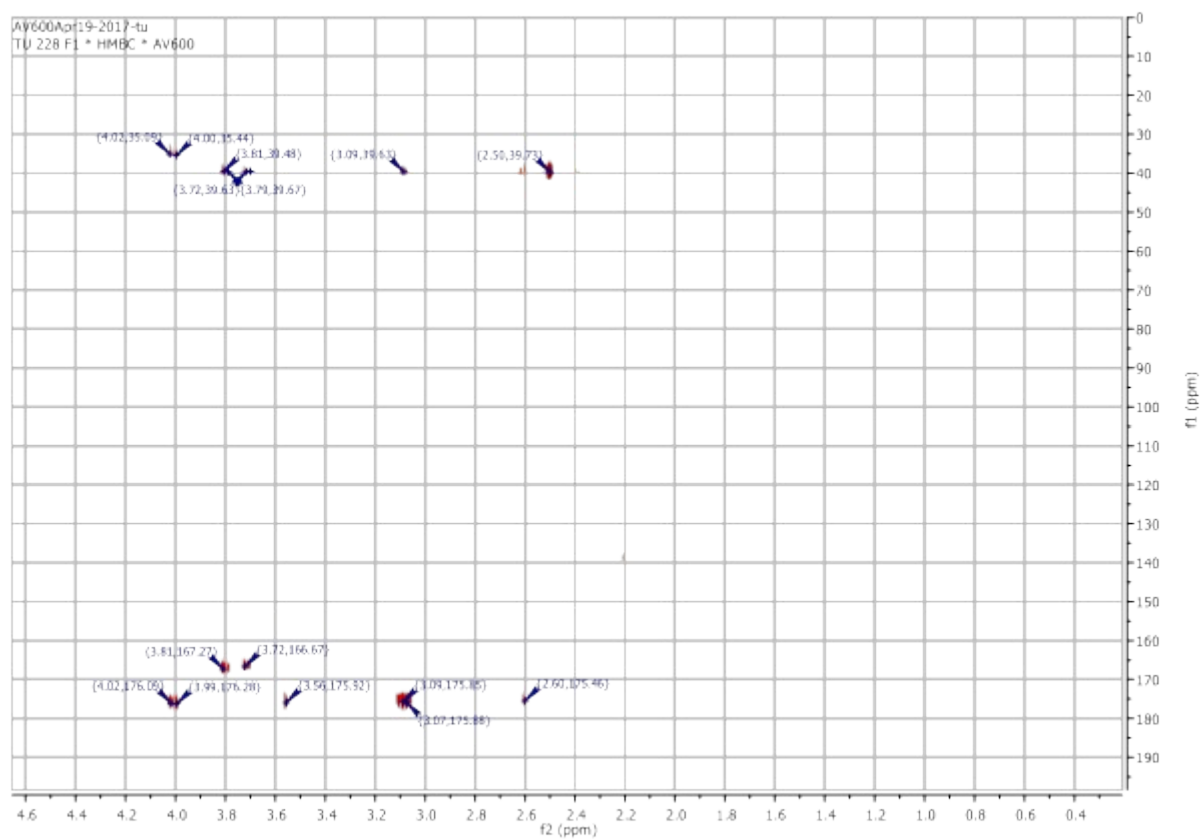
Figure 16: HMBC spectrum of PIS-3.
