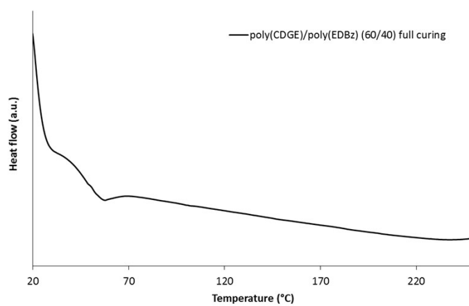
Figure 2. DSC analysis (N 2 , 20 °C/min) of the (60/40) poly(CDGE)/poly(EDBz) IPN after the full curing.
