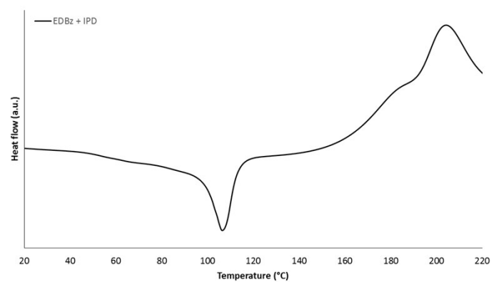
Figure 1. DSC analysis (N 2 , 20 °C/min) of EDBz in presence of IPD.
