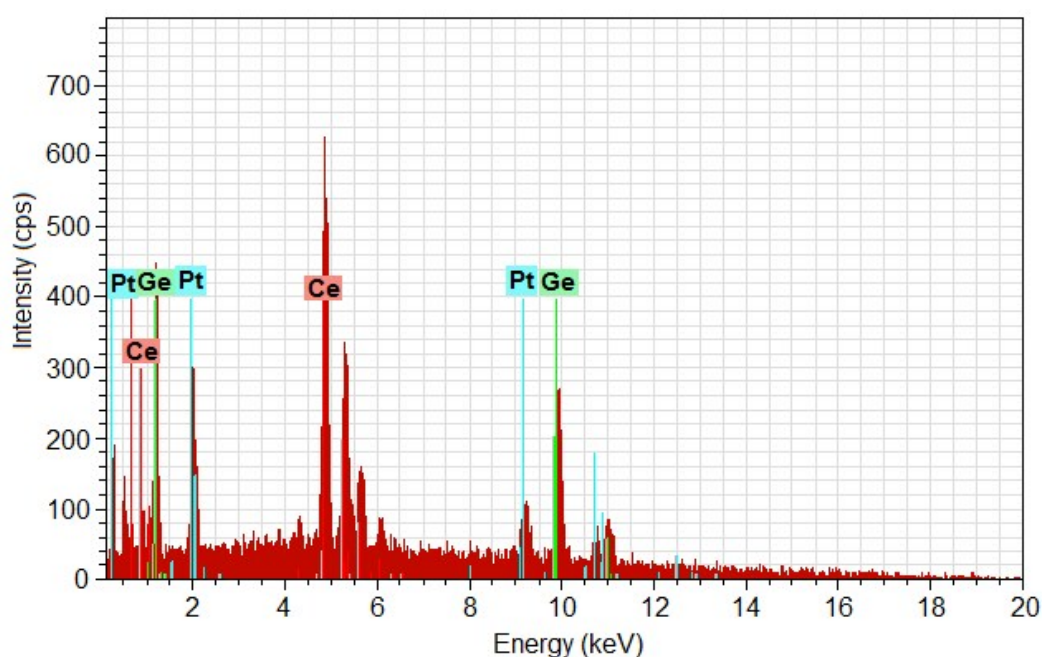
Figure S1 Energy Dispersive X-ray absorption (EDX) spectrum on Ce 2 PtGe 3 sample.
