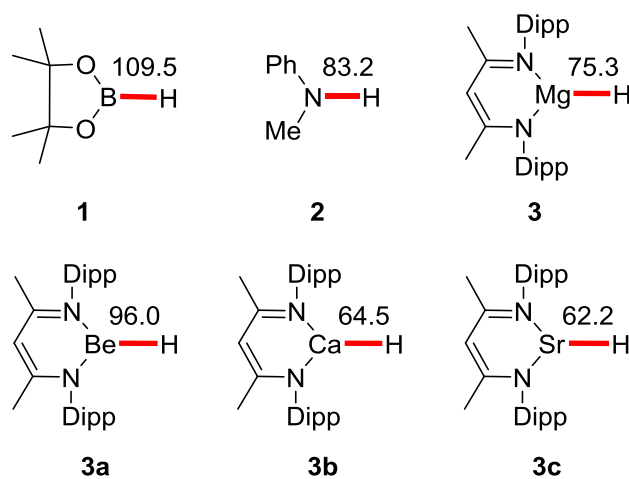
Fig. S1. The value of BDEs. The BDEs are given in kcal/mol.
