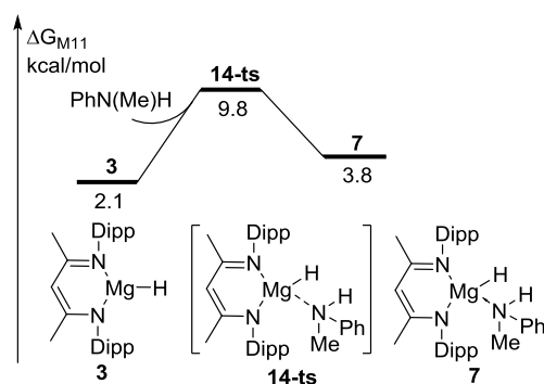
Fig. S2 Free energy profiles for the intermediate 3 to 7.
