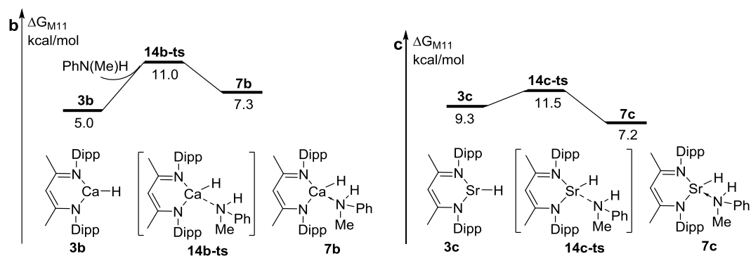
Fig. S3 Free energy profiles for the intermediate 3b to 7b(b) and 3c to 7c(c).
