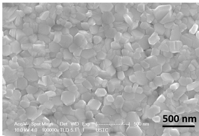
Figure S1 Surface sectional SEM images of the perovskite films fabricated by CP methods.
