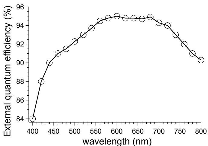
Figure S3. External quantum efficiency of the utilized Si-PV cell
