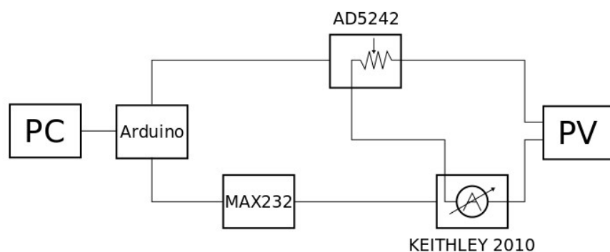
Figure S1. Scheme of the apparatus utilized for the photocurrent measurement
