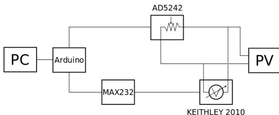
Figure S2. Scheme of the apparatus utilized for the voltage measurement
