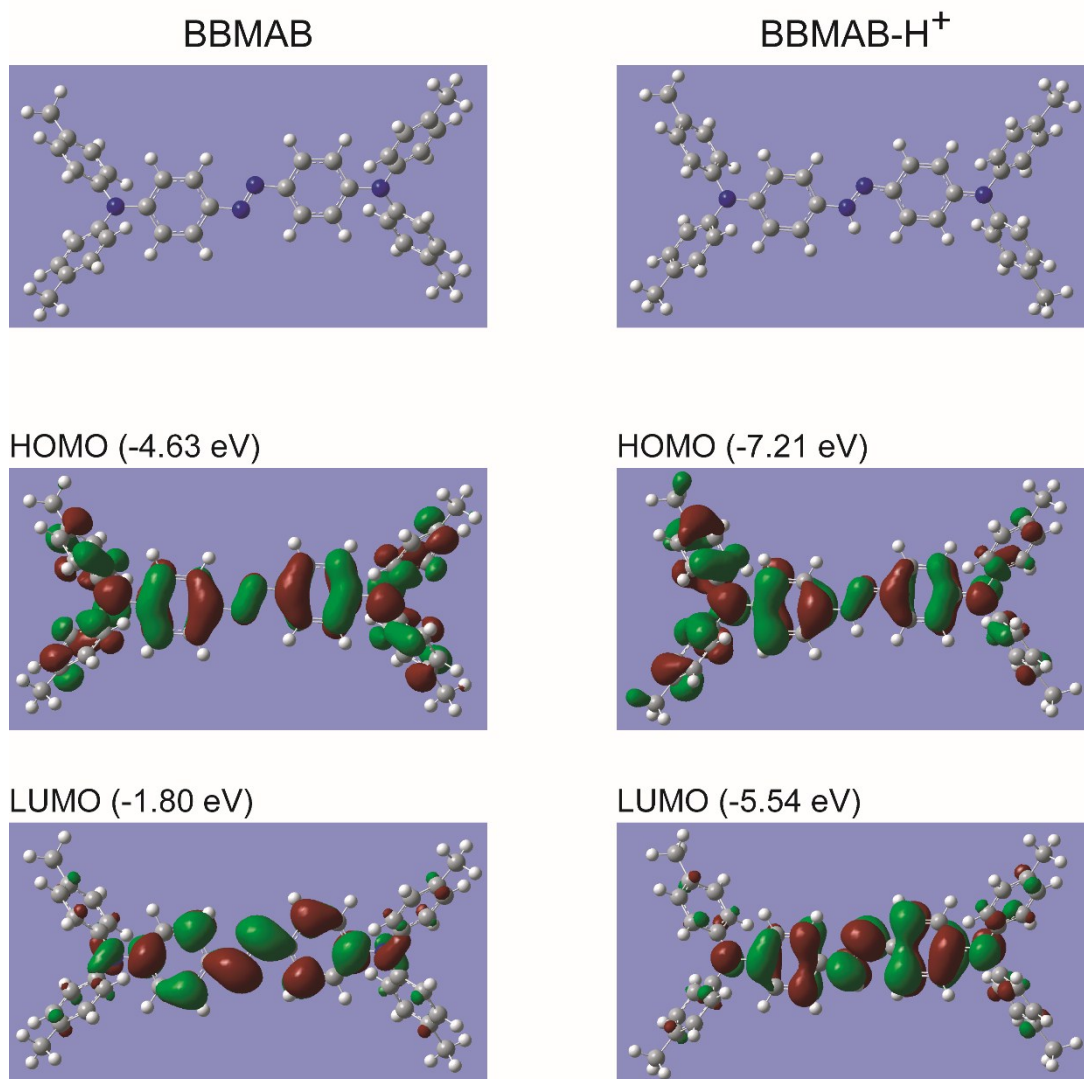
Fig. S1 Optimized molecular structures together with their HOMO and LUMO surfaces of BBMAB and BBMAB-H + obtained by DFT calculation (B3LYP/6-31G(d,p))
