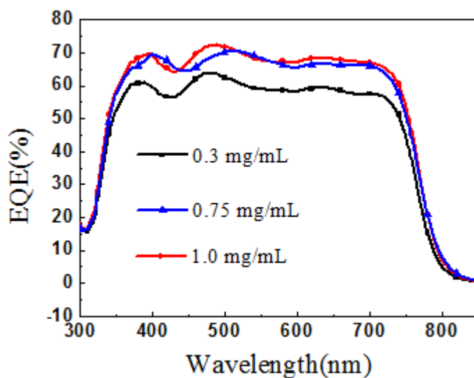
Figure S2. The EQE of the photodetectors with the ITO modification by different concentration of WC-2 solution.
