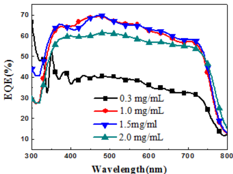
Figure S1. The EQE of the photodetectors with the ITO modification by different concentration of WC-1 solution.
