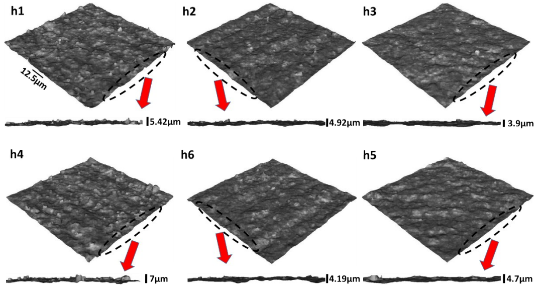
Fig. S1. 3D view images of resulting surface topographies were captured by Alicona system.
