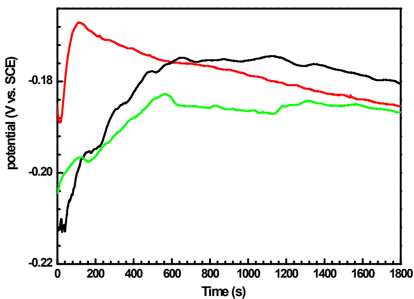
Fig. S1 The open circuit potential versus time of PDA@Cu samples recorded in 3 wt.% NaCl aqueous solution for three times.
