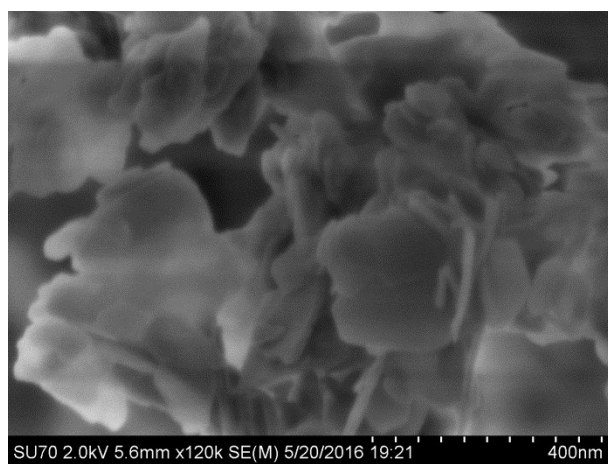
Fig. S2 SEM image of reduced catalyst PtSn/Mg(2-Ga)AlO
