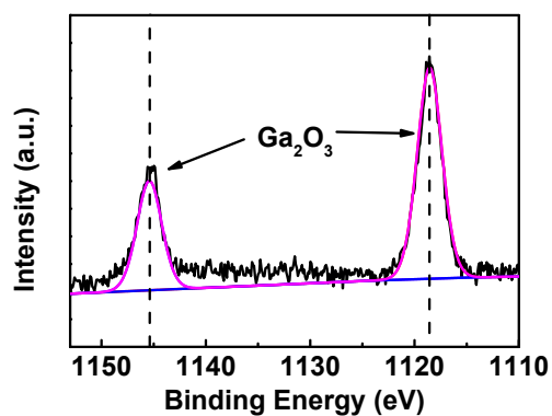
Fig. S1 The XPS spectra of Ga2p for PtSn/Mg(2-Ga)AlO catalyst
