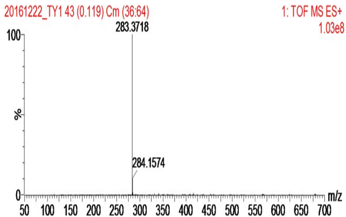
Figure S3. The HRMS spectrum of 1 .
