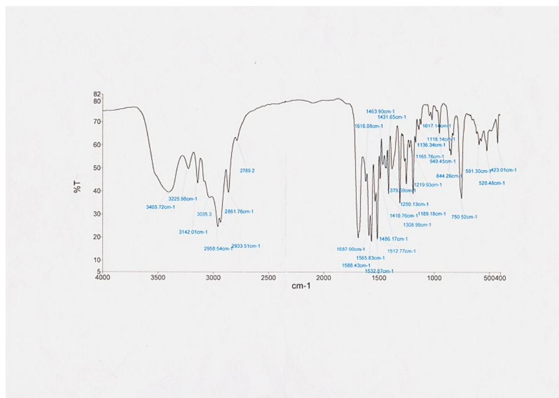
Figure S4. The FTIR spectrum of 1 .
