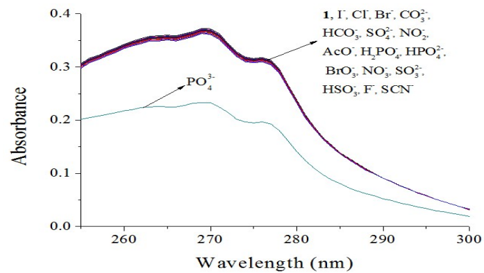
Figure S5. UV-vis absorption spectra of probe 1 (10 \mu\text{M} ) upon addition of different anions (1.0 equiv.) in HEPES buffer (10 mM, pH 7.4, 25 ^{\circ}\text{C} ) solution.
