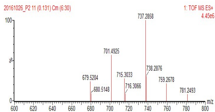
Figure S6. The HRMS spectrum of mixture of 1 with \text{PO}_4^{3-} .
