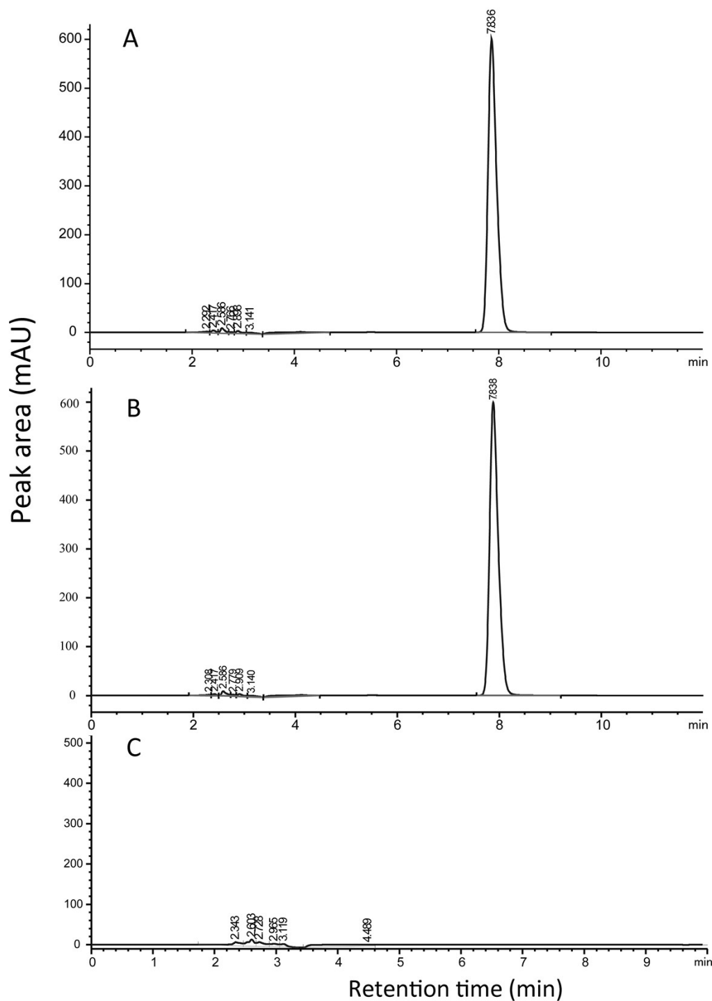
Figure S1 HPLC analysis of AAP biodegradation by resting cells of E. coli -pET28a.
