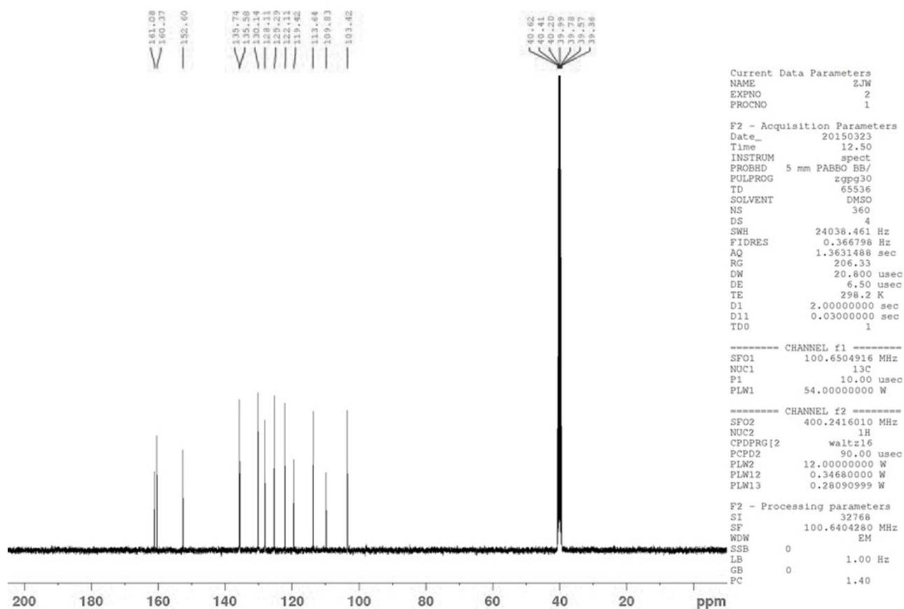
Fig. S4 13 C NMR spectra of UroB.
