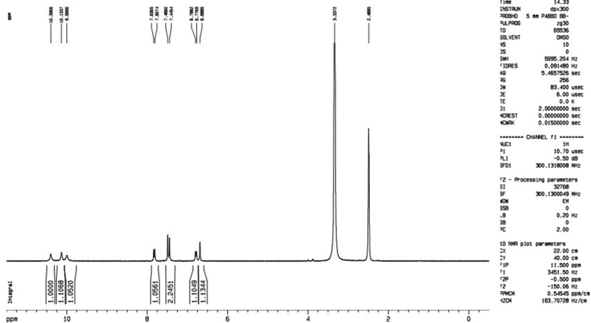
Fig. S5 ^1\text{H} NMR spectra of UroC.
