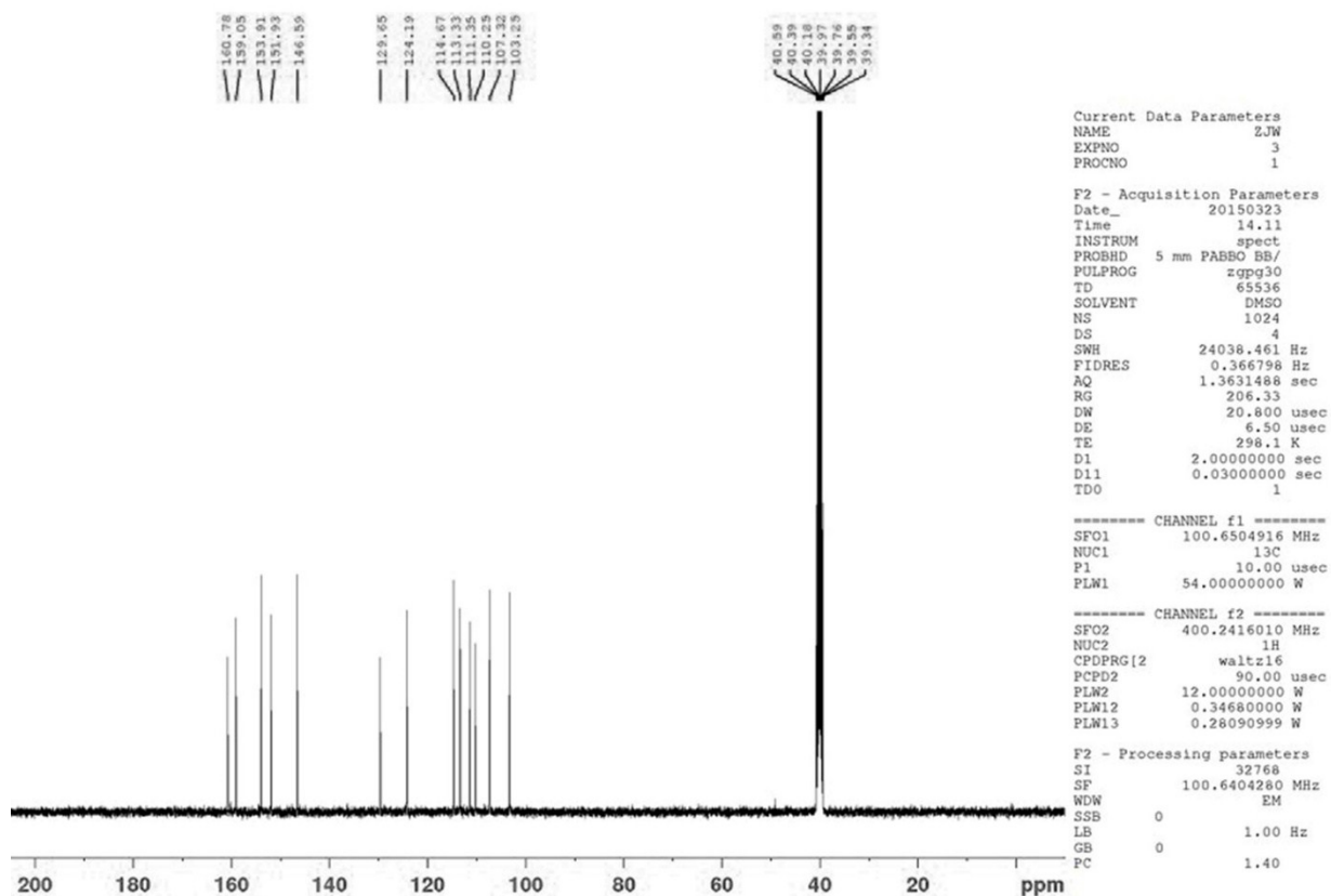
Fig. S6 ^{13}\text{C} NMR spectra of UroC.
