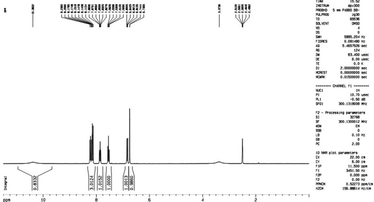
Fig. S3 1 H NMR spectra of UroB.
