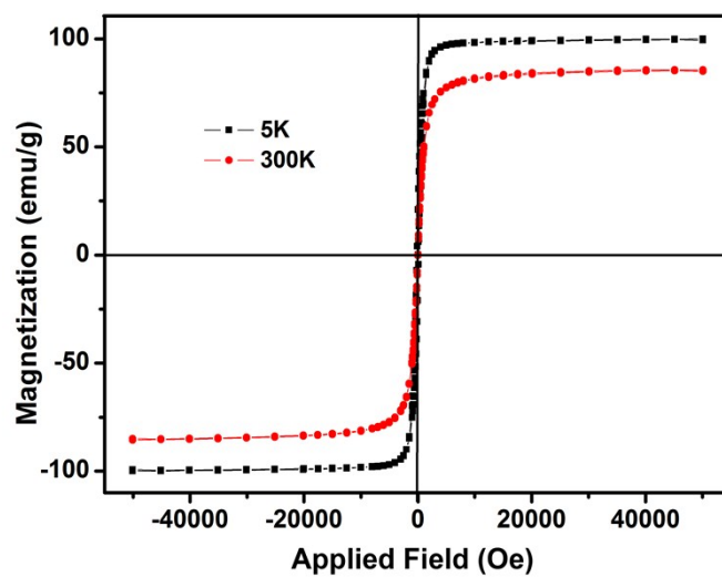
Fig. S2 The field-dependent magnetization curve (M-H curve).
