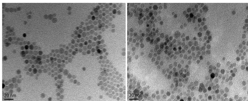
Fig. S1 TEM images of (a) Fe 3 O 4 -OA and (b) Fe 3 O 4 -TETT NPs.
