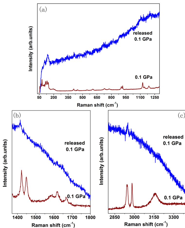
Figure S1. Raman spectra on compression at 0.1 GPa and decompression at 0.1 GPa, ranging from 50-3500 \text{cm}^{-1} , respectively. After released, the fluorescence of malonamide enhanced significantly.
