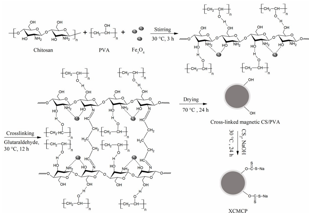
Fig. S1. Schematic illustrations of the synthesis strategy used to prepare xanthate-modified cross-linked magnetic chitosan/poly (vinyl alcohol) particles
