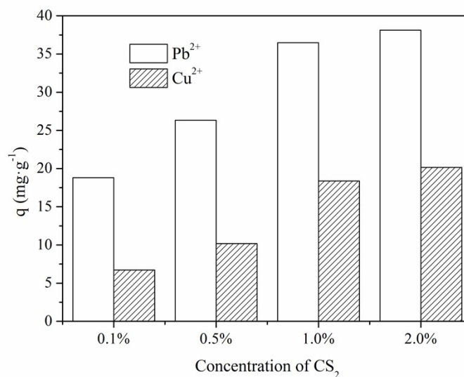
Fig. S2. Effect of CS_2 on adsorption of Pb^{2+} and Cu^{2+} onto XCMCP. Experimental condition: initial metal ions concentration was 100 mg/L, dosage of XCMCP was 0.15 g/ 50 mL, and temperature was 303K
