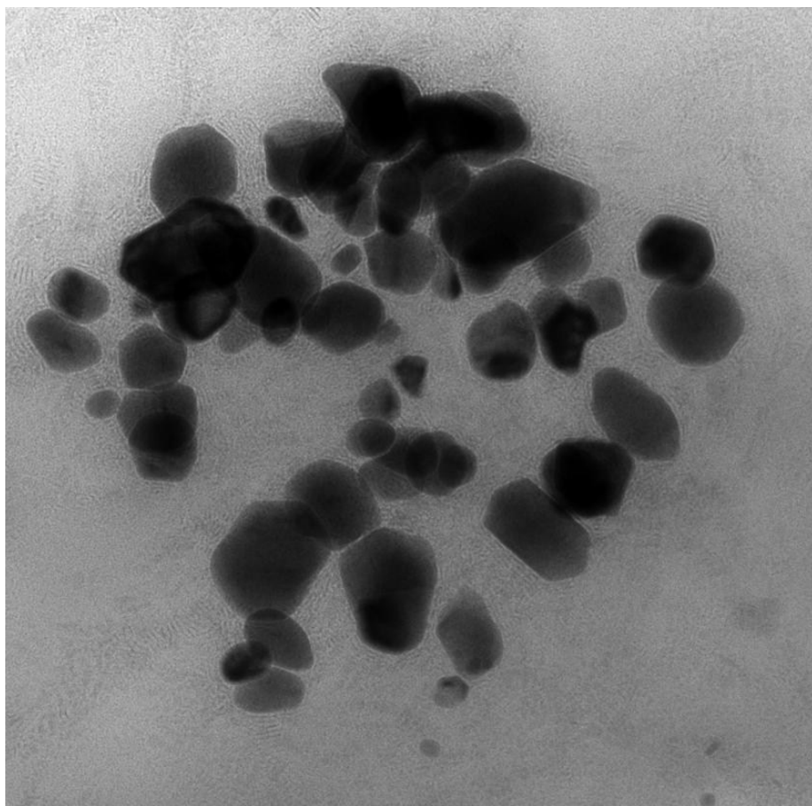
Figure S1: TEM image of In nanoparticles synthesized without controlling the rate of addition of \text{NaBH}_4 .
