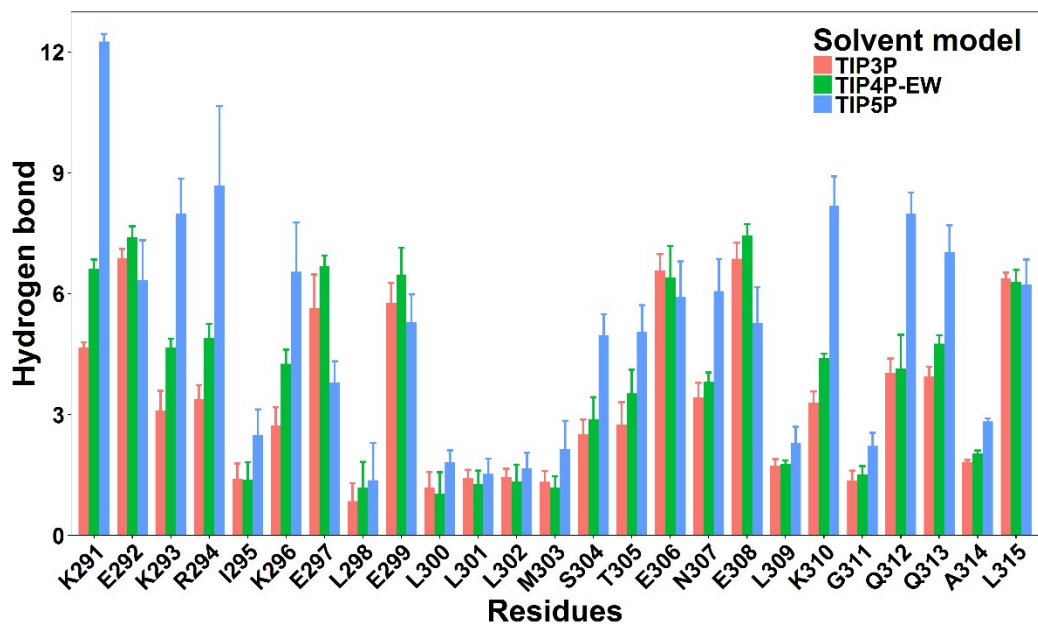
Figure S1. Hydrogen bond between water and c-Myb for different solvent models.
