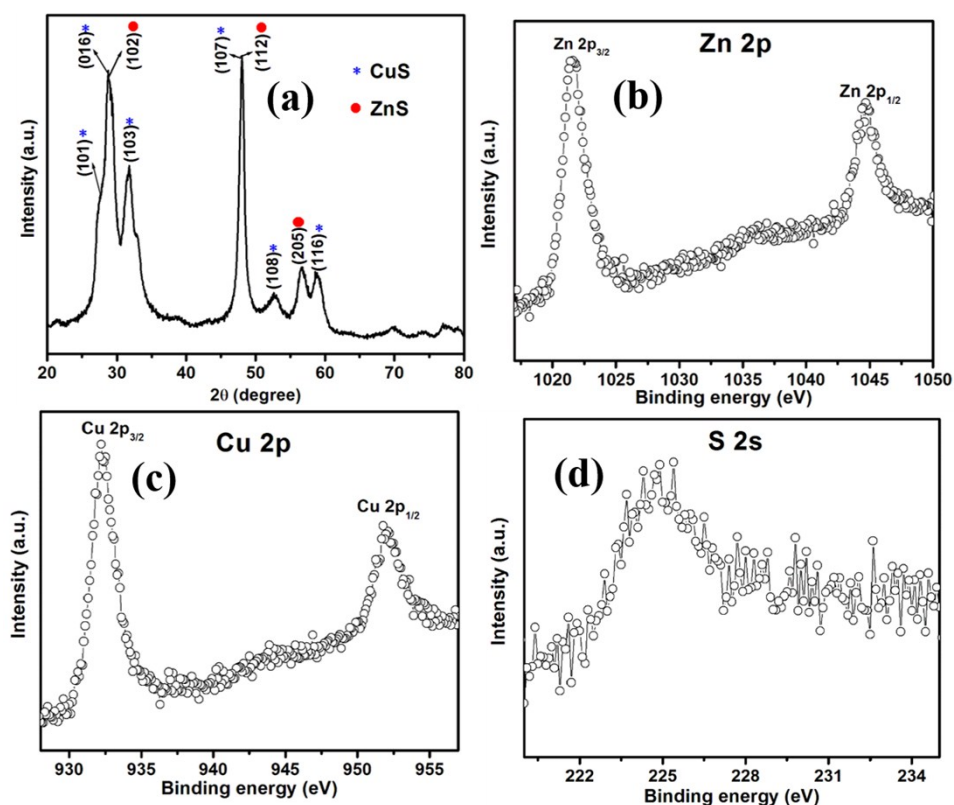
Fig. S1. XRD (a) and XPS spectra of (b) Zn 2p state, (c) Cu 2p state and (d) S 2s states of sample ZC2 after photocatalytic reaction.
