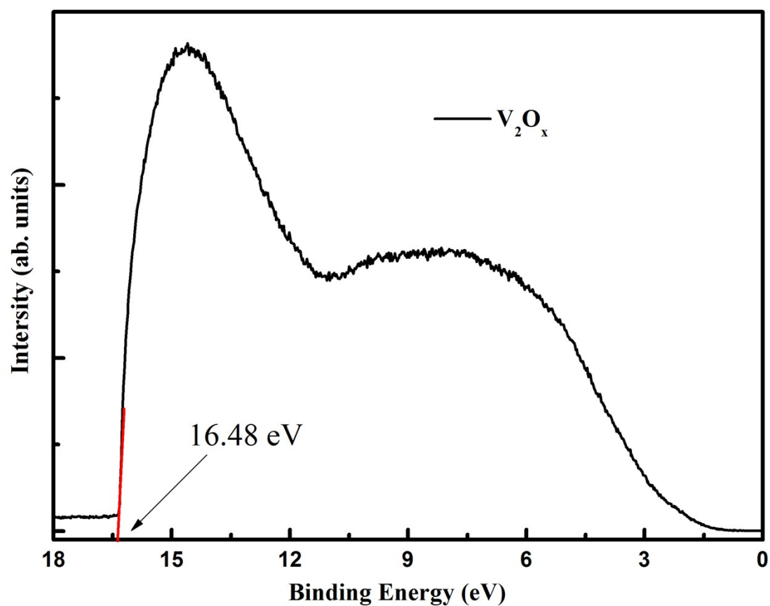
Fig. S1 The UPS spectra of V_2O_x film.
