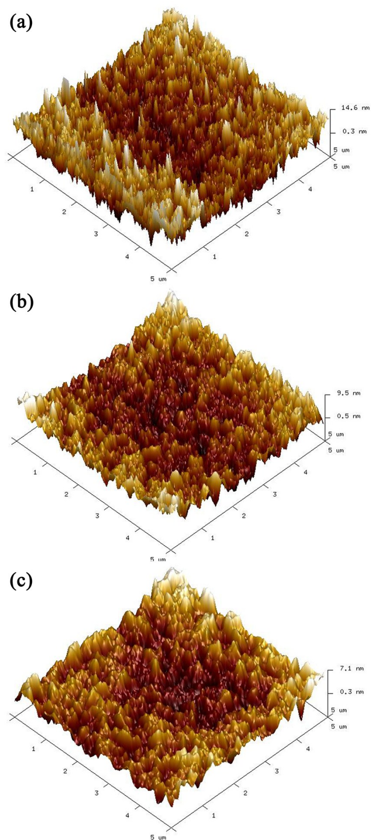
Fig. S2 3D AFM images of \text{V}_2\text{O}_x film (a), PEDOT:PSS film (b), and \text{V}_2\text{O}_x/\text{PEDOT:PSS} film (c) based on ITO coated glasses.
