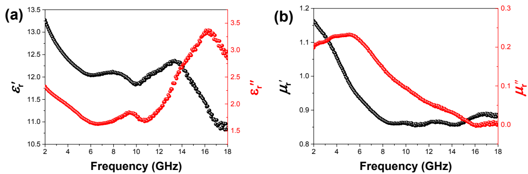
Fig. S1. The complex permittivity and permeability of Ni/C-paraffin composites.
