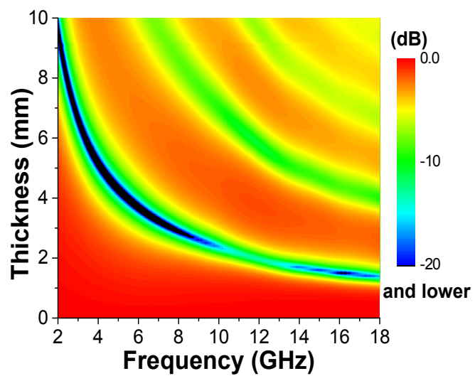
Fig. S2. The two-dimensional (2D) plot of microwave absorption ( RL ) of the Ni/C-paraffin composites.
