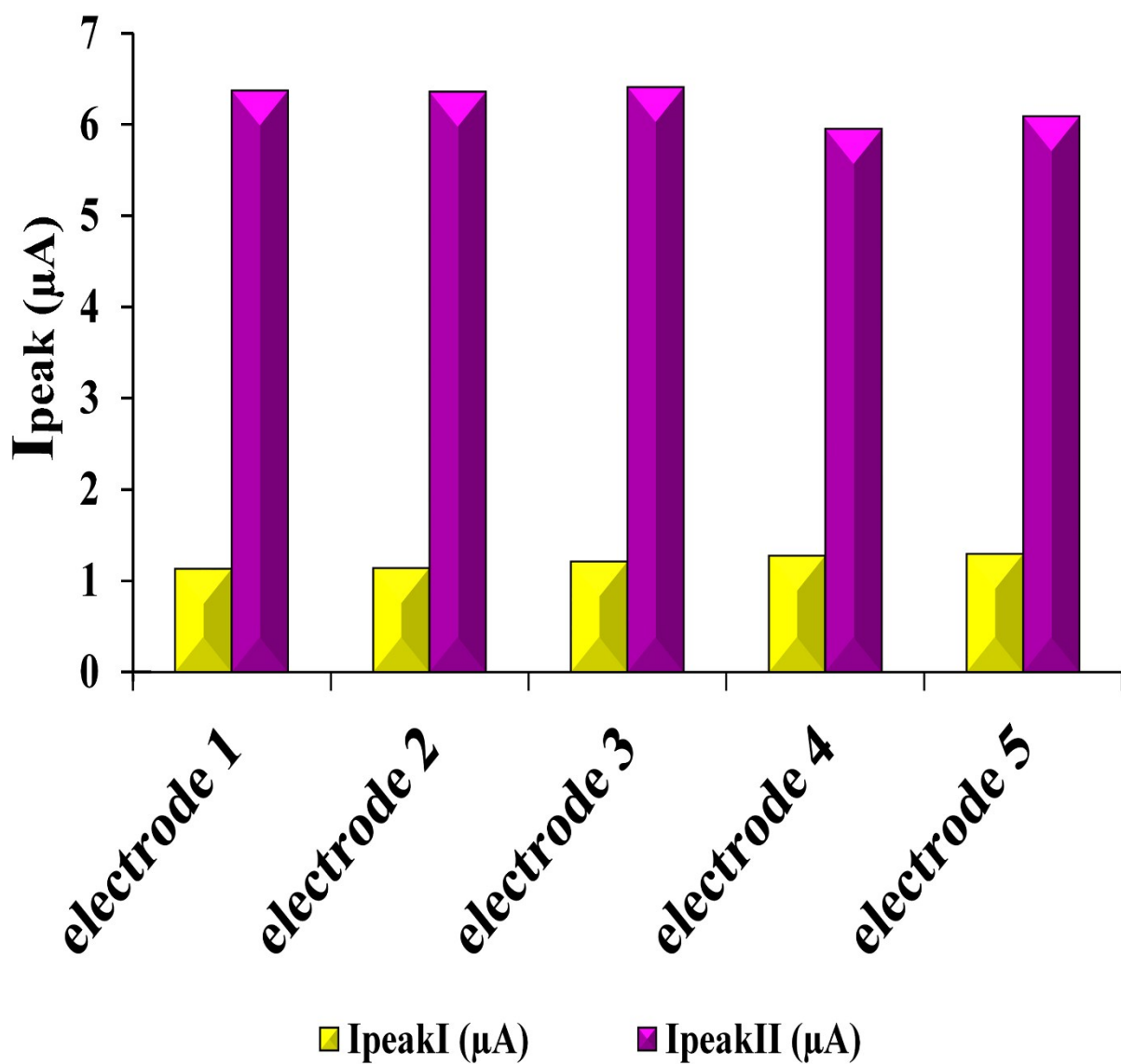
Fig S2. Reproducibility of the modified electrode in 5.0 \mu M RIF
