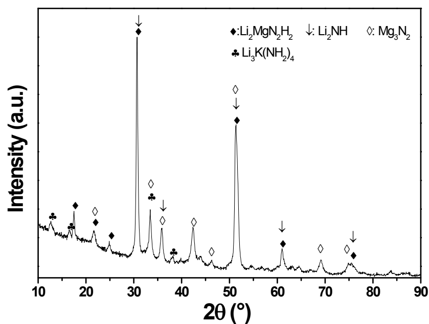
Fig. S1 XRD pattern of the \text{LiNH}_2\text{-Li}_2\text{Mg}_2\text{N}_3\text{H}_3\text{-0.84LiH-0.16KH} sample dehydrogenated at 280 °C.
