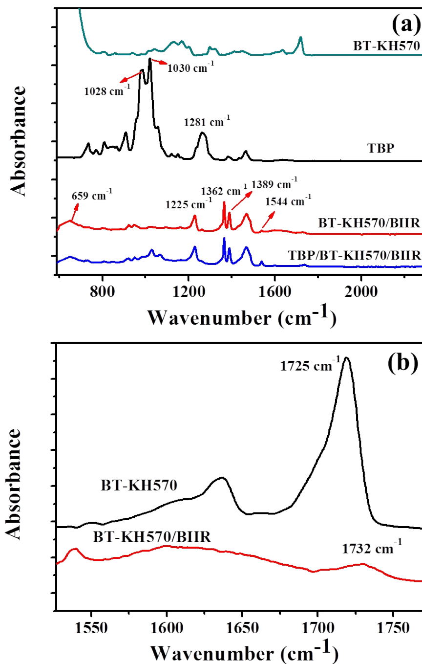
Fig.S1 FTIR spectra of (a) BT-KH570, TBP, 10 phr BT-KH570/BIIR, 30 phr TBP/(10 phr BT-KH570/BIIR) composite in the wavenumber range 584 \text{cm}^{-1} to 2300 \text{cm}^{-1} , (b) BT-KH570, 10 phr BT-KH570/BIIR composite in the wavenumber range 1527 \text{cm}^{-1} to 1770 \text{cm}^{-1} .
