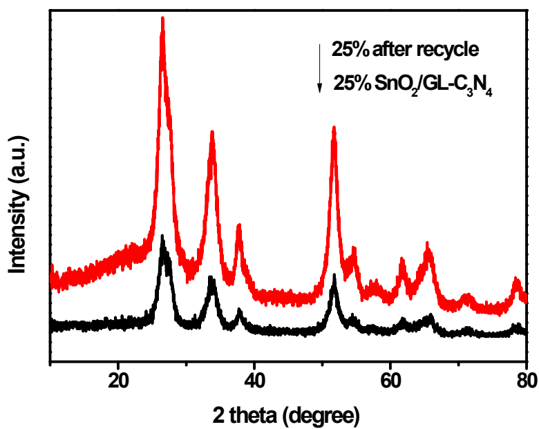
Fig. S1 XRD patterns of 25 wt% GL-SnO 2 /C 3 N 4 composites.
