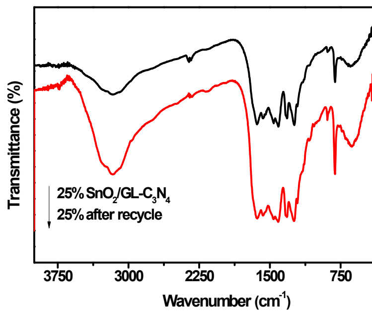
Fig. S2 FT-IR patterns of 25 wt% GL- \text{SnO}_2/\text{C}_3\text{N}_4 composites.
