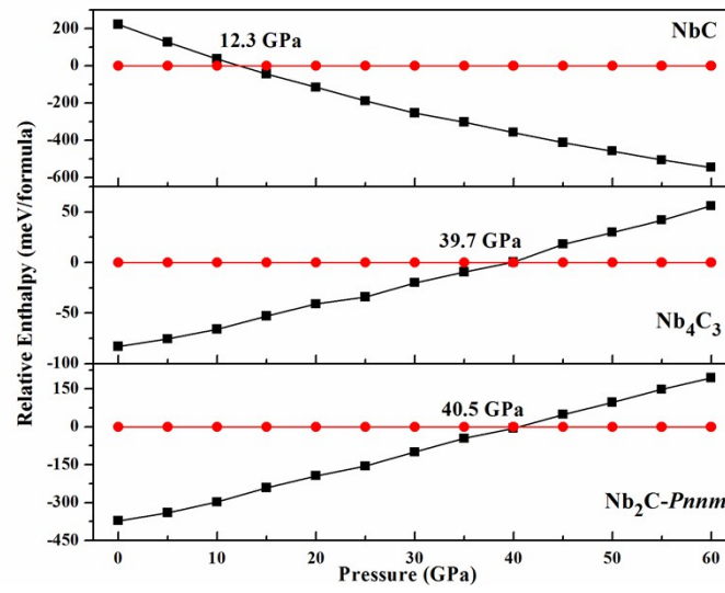
Figure SI | Calculated enthalpies as the function of pressure.
