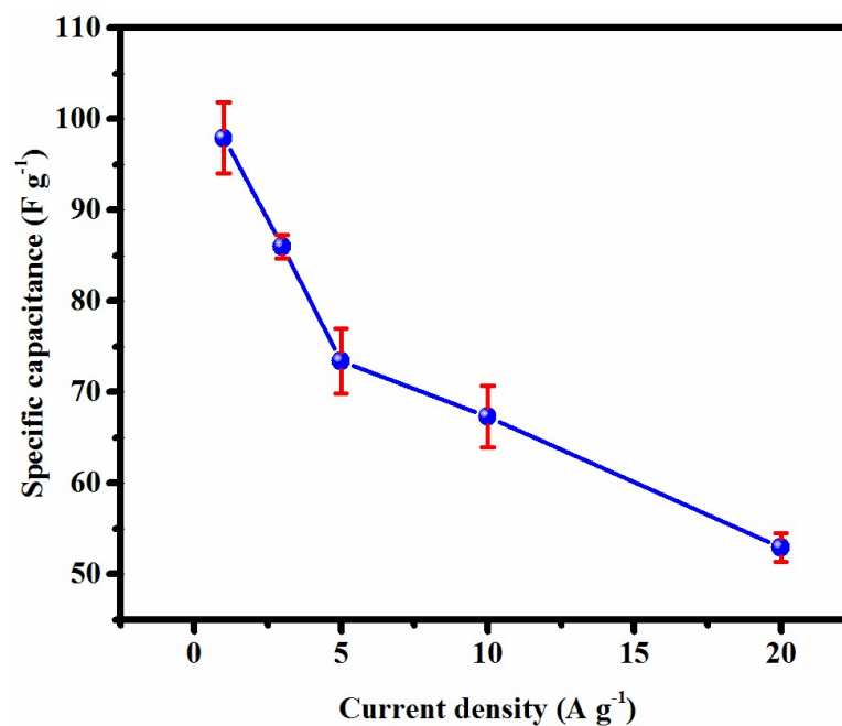
Fig. S2 Rate capability at various current densities ranging from 1 A g -1 to 20 A g -1 .
