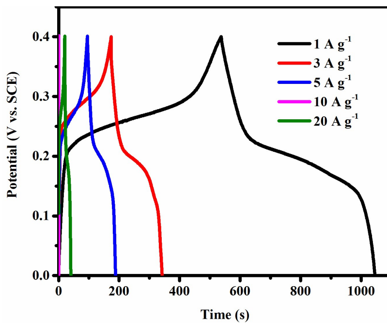
Fig. S1 GCD curves of NiO/NF at various current densities.
