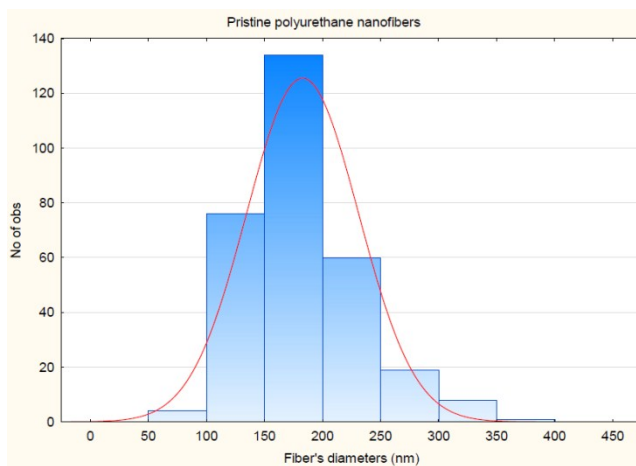
Figure 1s. Diameter distribution of pristine PU nanofibers
