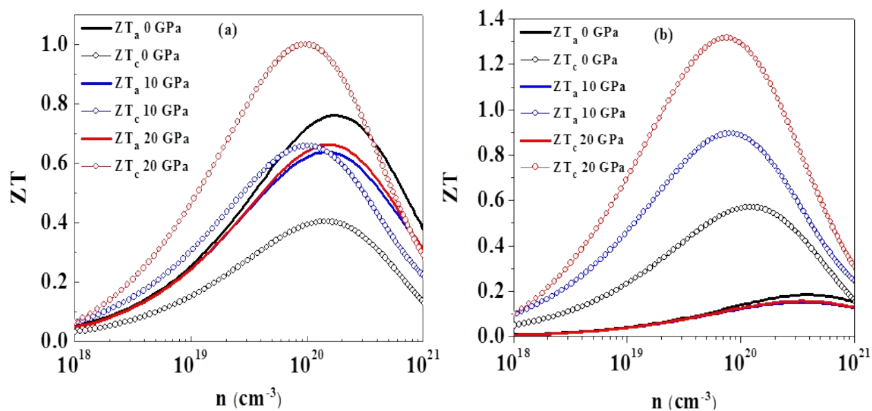
Figure S1 Figure of merit (ZT) studied in a and c directions at 800 K at 0 GPa, 10 GPa and 20 GPa; \kappa_l values taken from (a) Reference (3) (b) Reference (74)
