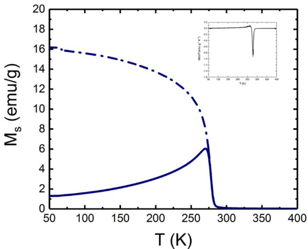
Fig. S1 Representation of Curie temperature T_C calculation. This is achieved by taking the derivative of ZFC curve.
