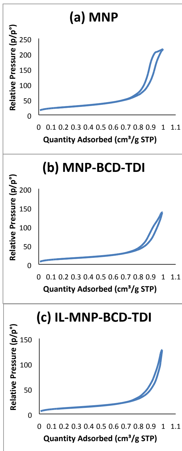
Fig. SI2 N 2 -adsorption/desorption isotherm (a) MNP, (b) MNP- \beta CD-TDI, and (c) IL-MNP- \beta CD-TDI
