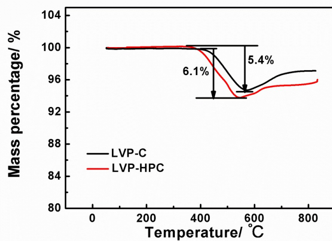
Fig. S2. TG curves of the LVP-C and LVP-HPC
