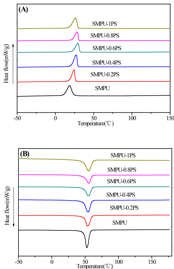
Figure S1. The DSC curves of MDEA based ZSMPUs (A- the cooling curves; B-the second DSC heating curves)
