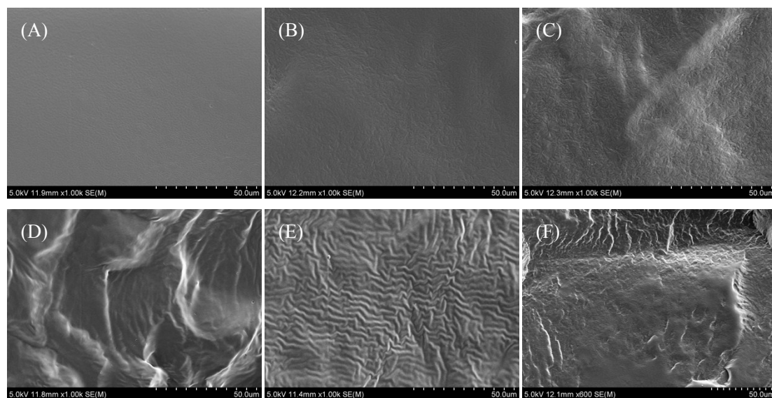
Figure S2. SEM images of MDEA based ZSMPUs (A-SMPU, B-SMPU-0.2PS, C-SMPU-0.4PS, D-SMPU-0.6PS, E- SMPU-0.8PS, F- SMPU-1.0PS)
