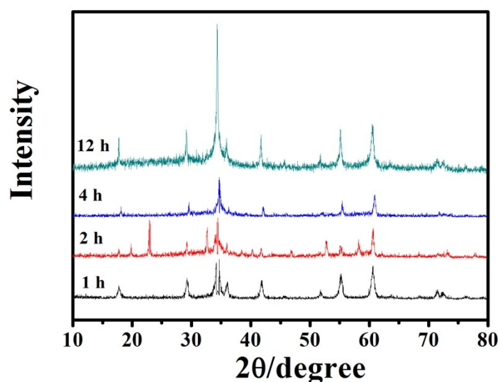
Fig. S1. The XRD patterns of the Zn 2 SnO 4 microspheres synthesized at different hydrothermal time
