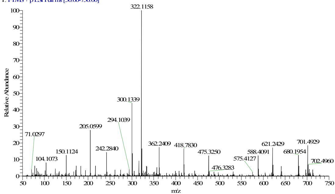
Fig. S3 The HRMS of L
