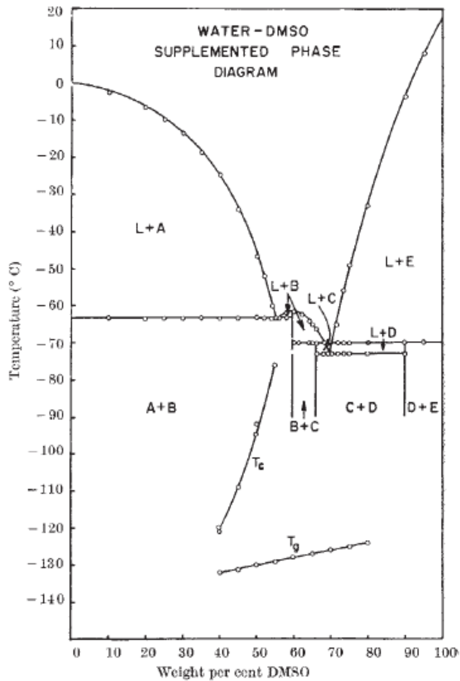
Figure S3: Phase diagram for DMSO-water binary mixture
