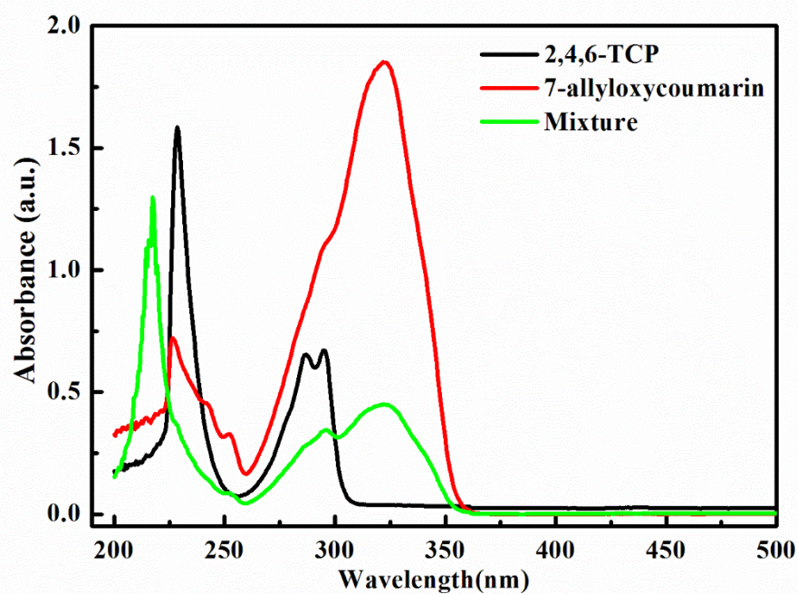
Figure S2. The absorption spectra of 2,4,6-TCP, 7-allyloxy coumarin and mixture solution in dichloromethane (a mixture of 2,4,6-TCP and 7-allyloxy coumarin in a molar ratio of 1:1).
