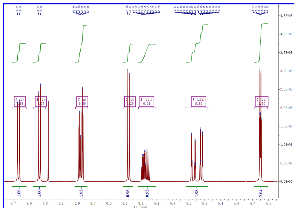
Figure S1. ^1\text{H} NMR of 7-allyloxy coumarin
