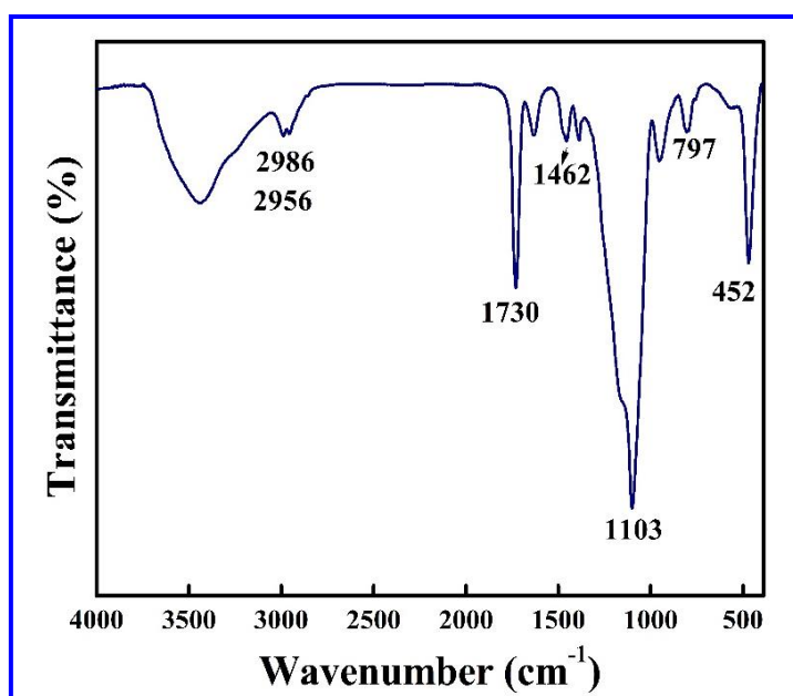
Figure S6. FT-IR spectra of SiO 2 @dye-FMIPs
