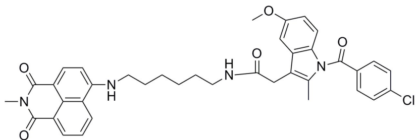
Supplementary Figure 1. The molecular structure of the COX-2 -specific fluorogenic probe.
