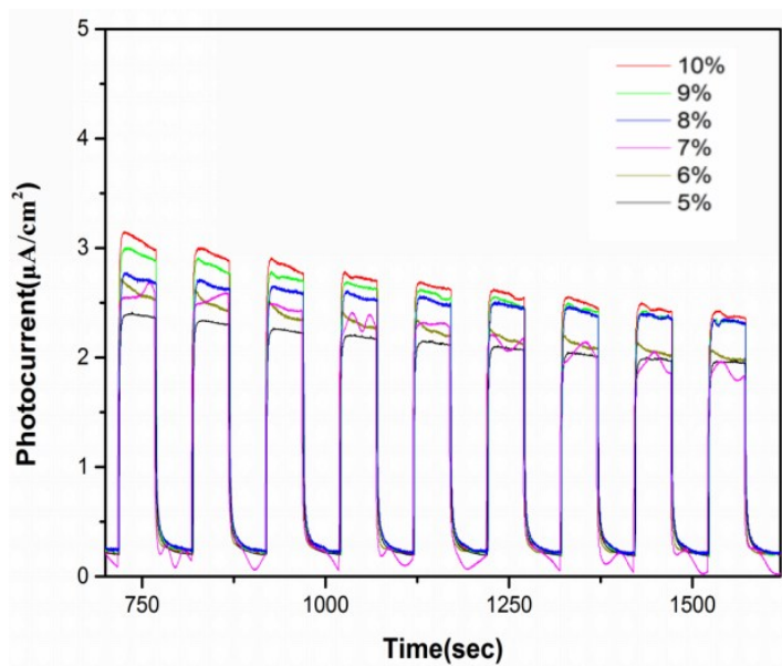
Fig. S2 Transient photocurrent response curve of 5%-10% (2Al, S) co-doped SnO 2 .
