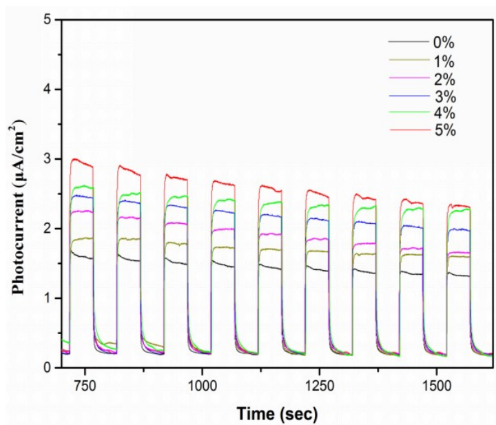
Fig. S1 Transient photocurrent response curve of 0%-5% (2Al, S) co-doped SnO 2 .
