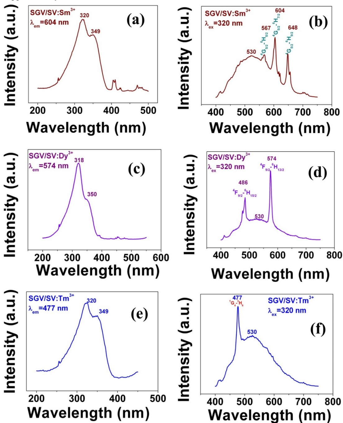
Figure S1. PL excitation and emission spectra of SGV/SV:Ln 3+ .(a) and (b): SGV/SV:Sm 3+ ; (c) and (d): SGV/SV:Dy 3+ ; (e) and (f):SGV/SV:Tm 3+ .
